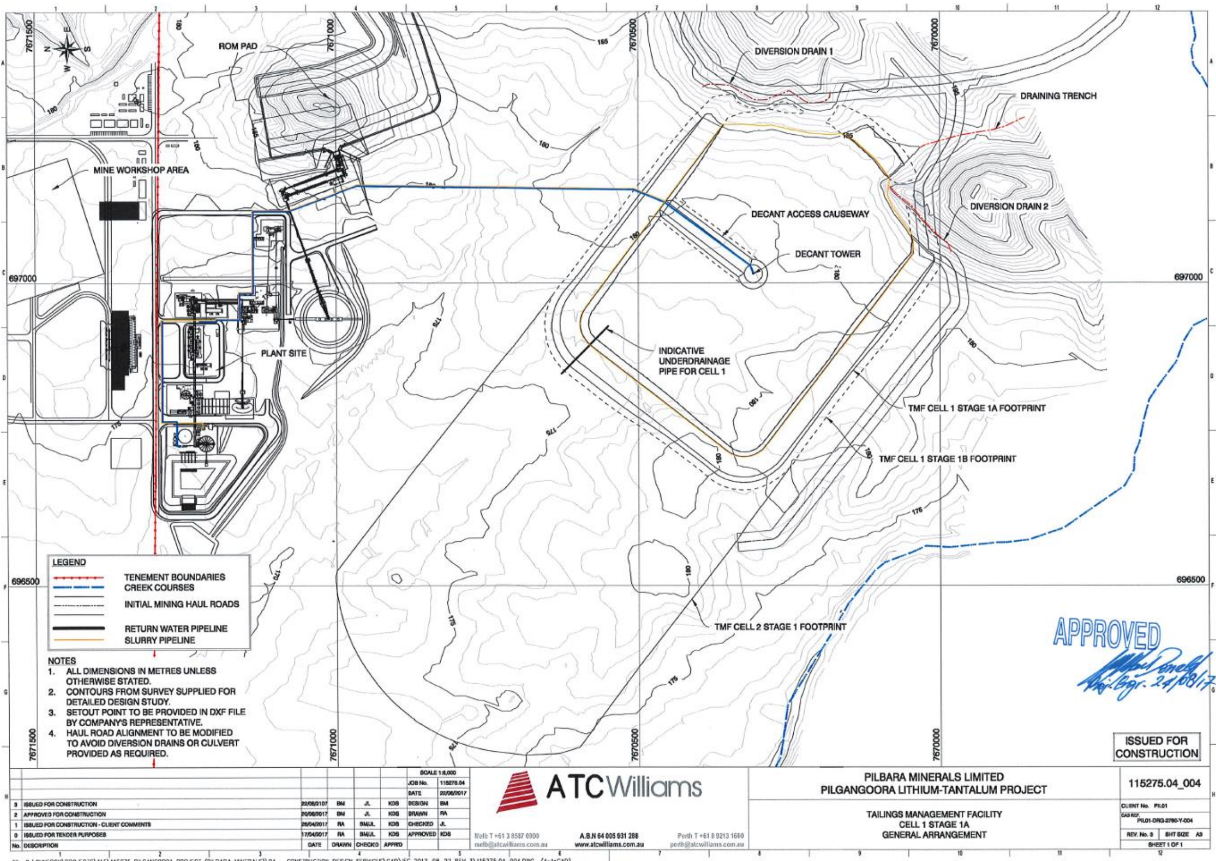
Site Plan 14: TMF 1 Tailings and Decant Pipeline Location and Location of underdrainage pipe
