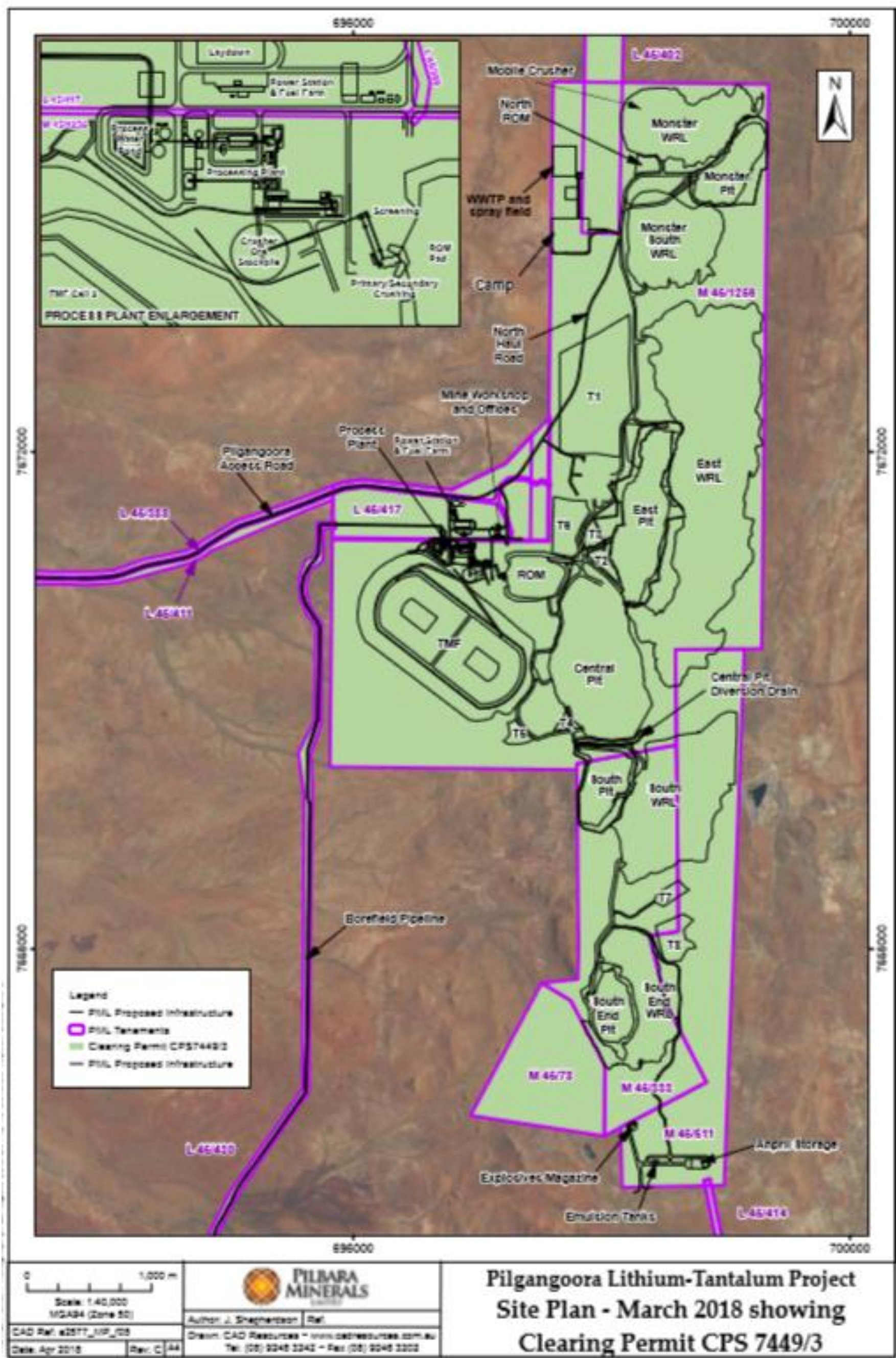
Site Plan 11: Initial mobile crusher location in Monster WRL
