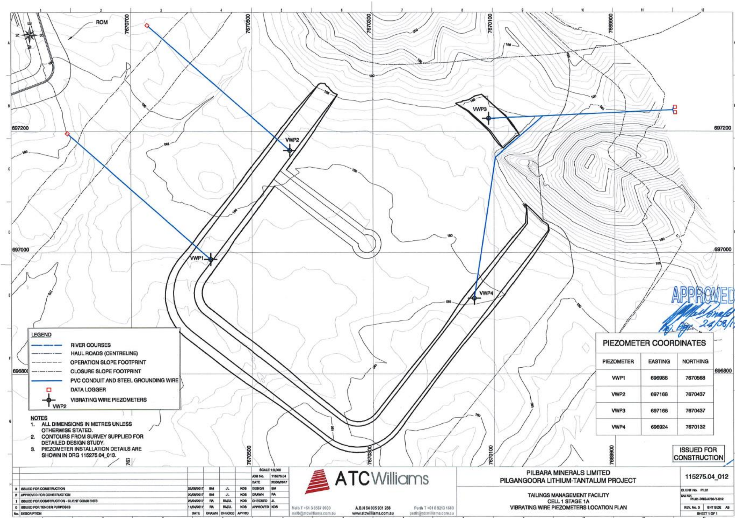
Site Plan 13: TMF 1 locations of VWP's (Stage 1A)
