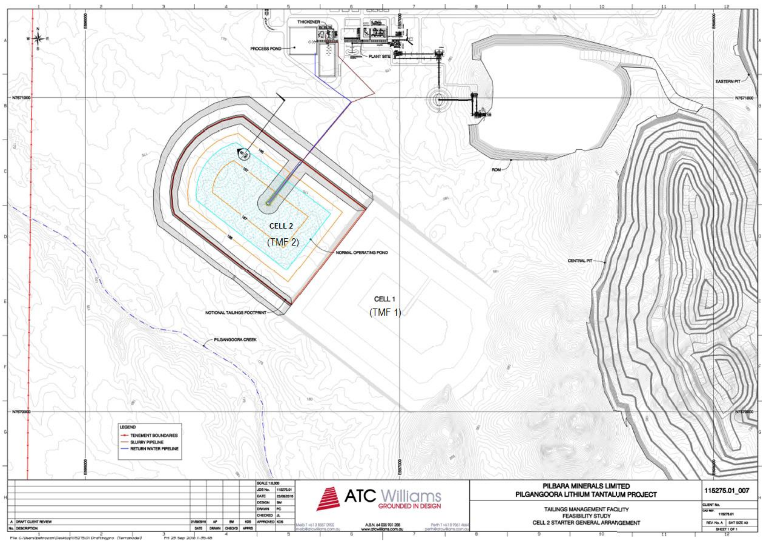
Site Plan 3: TMF general arrangement
