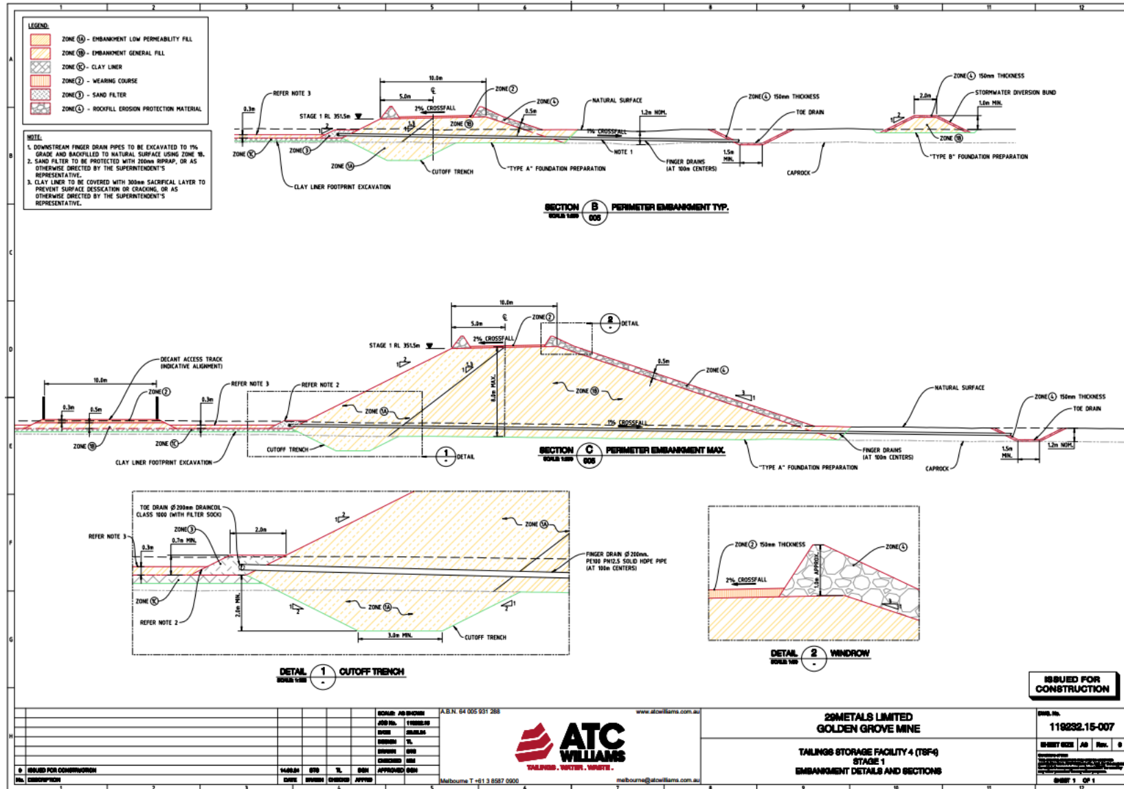
Figure 9: Design cross section of the TSF4 embankment
