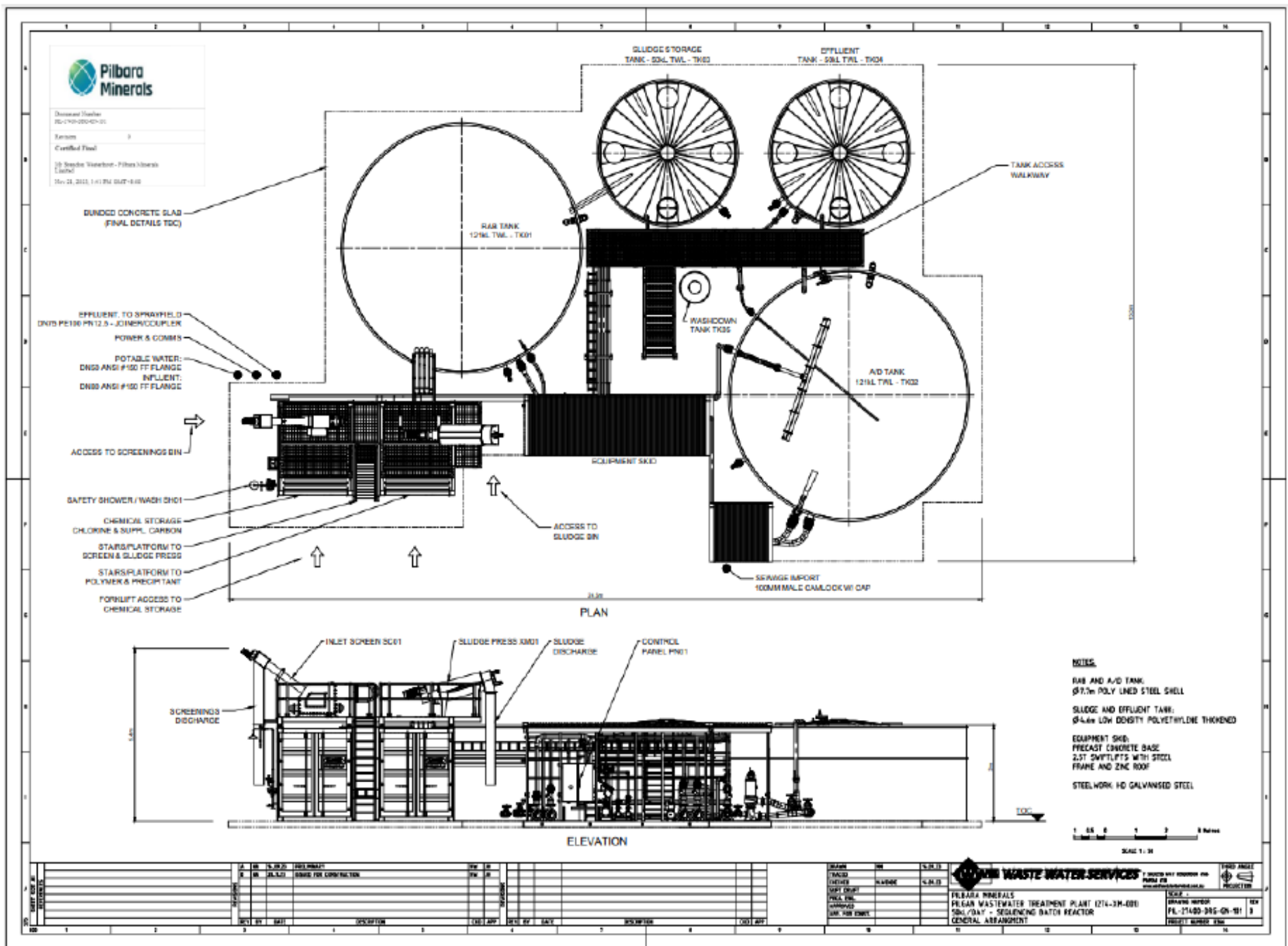
Figure 18: Pilbara Processing Plant WWTP General Arrangement
