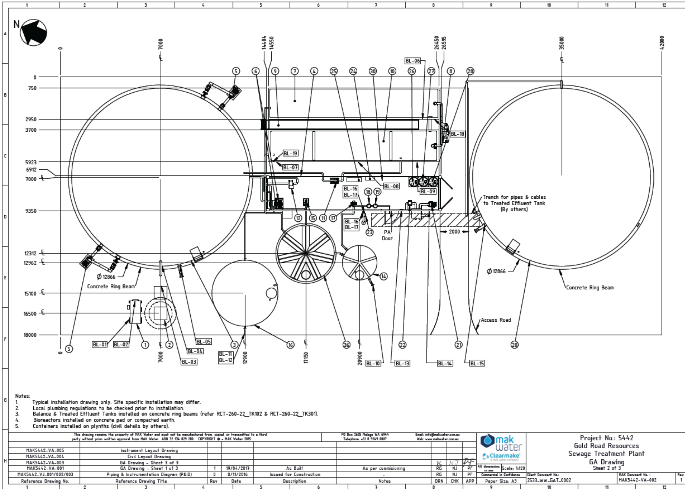
Figure 11: Stage 2 Temporary Construction Wastewater Treatment Plant
