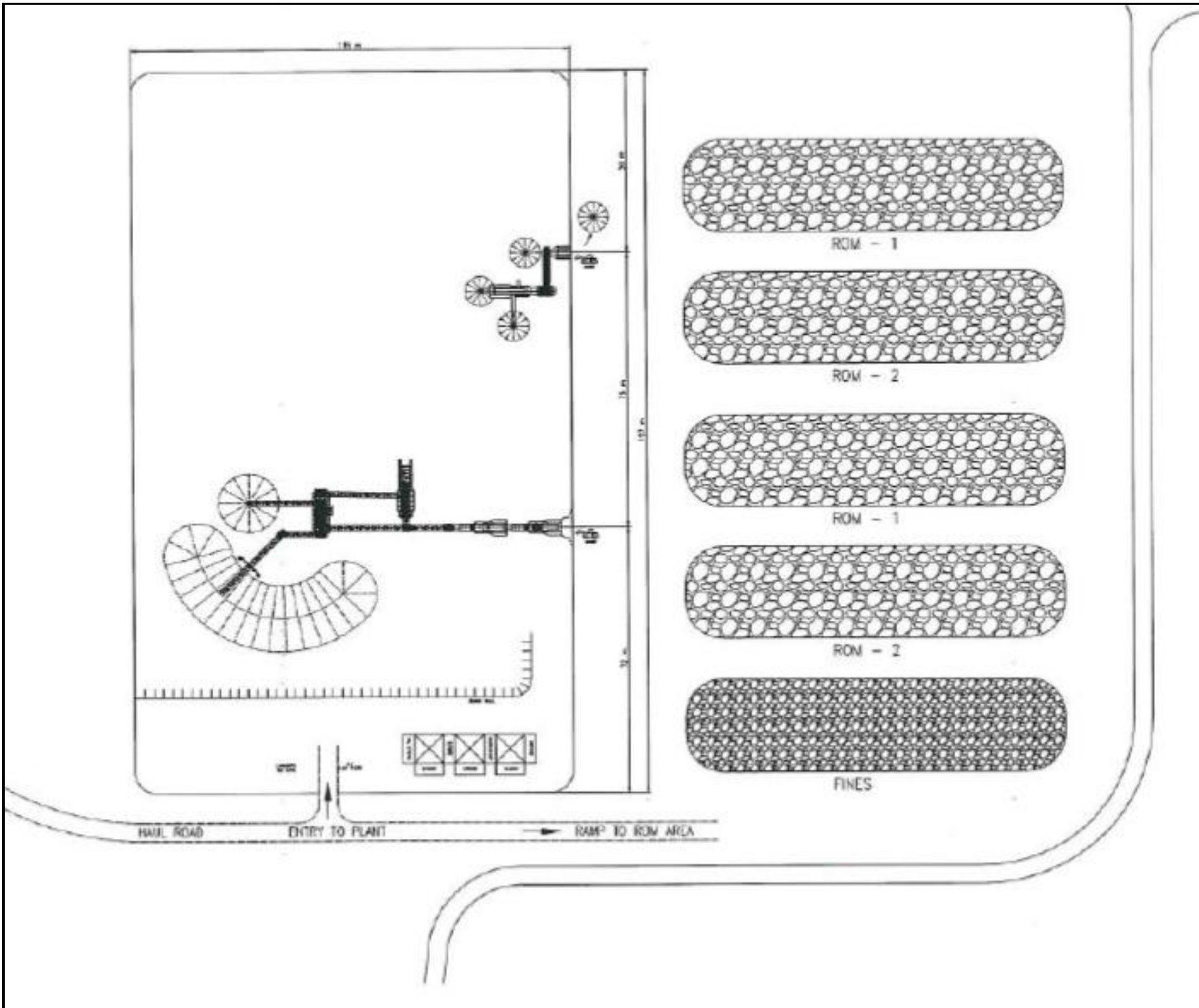
Figure 10: Initial mobile crushing and screening plant layout (for construction)
