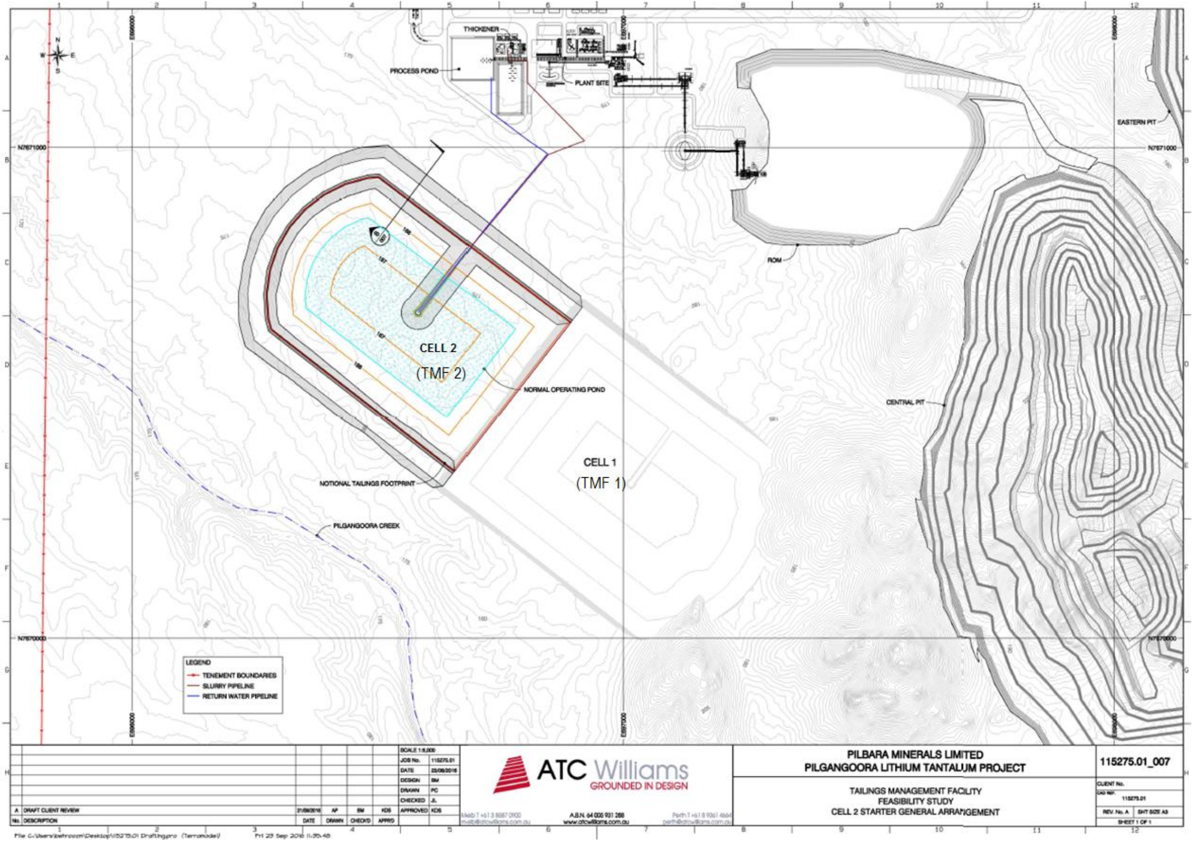
Figure 5: TMF general arrangement
