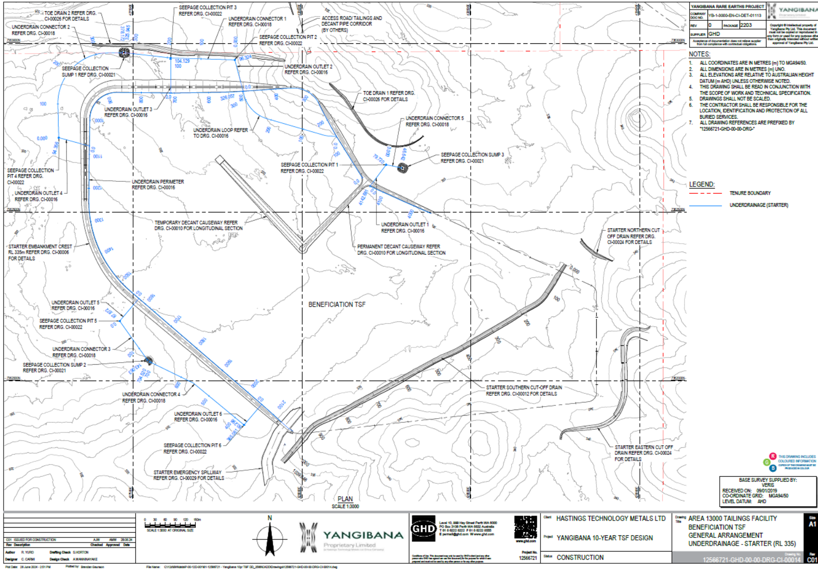
Figure 12: Underdrainage design
