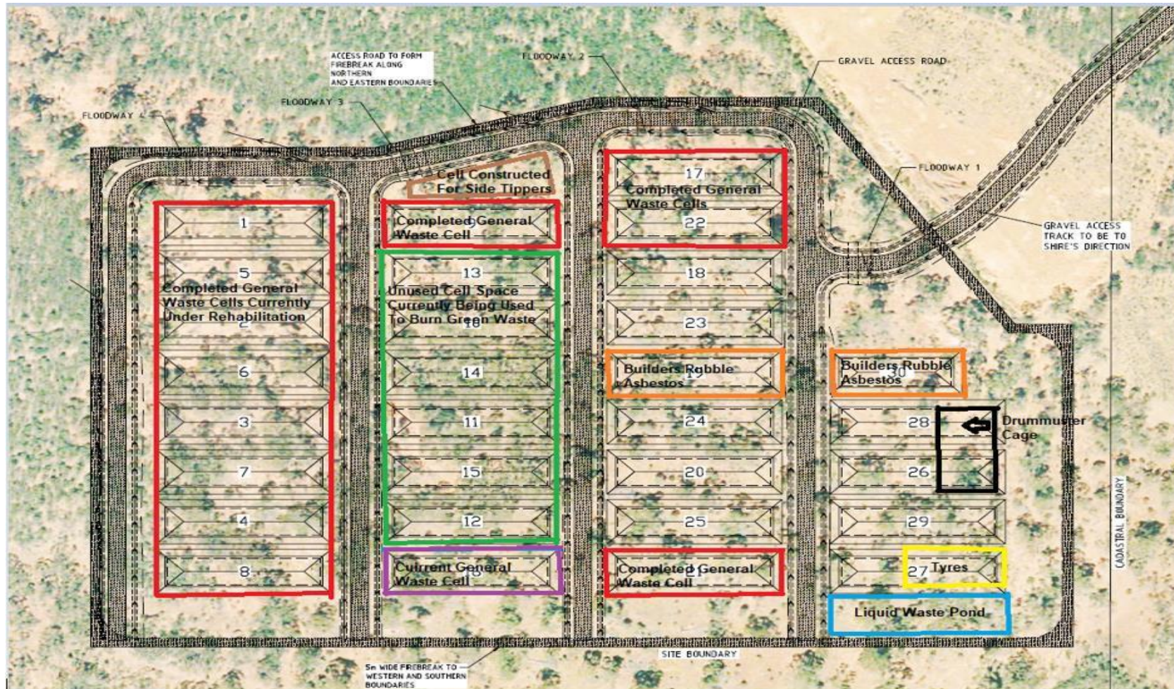
Figure 2: Current landfill layout and conceptual design within the premises
