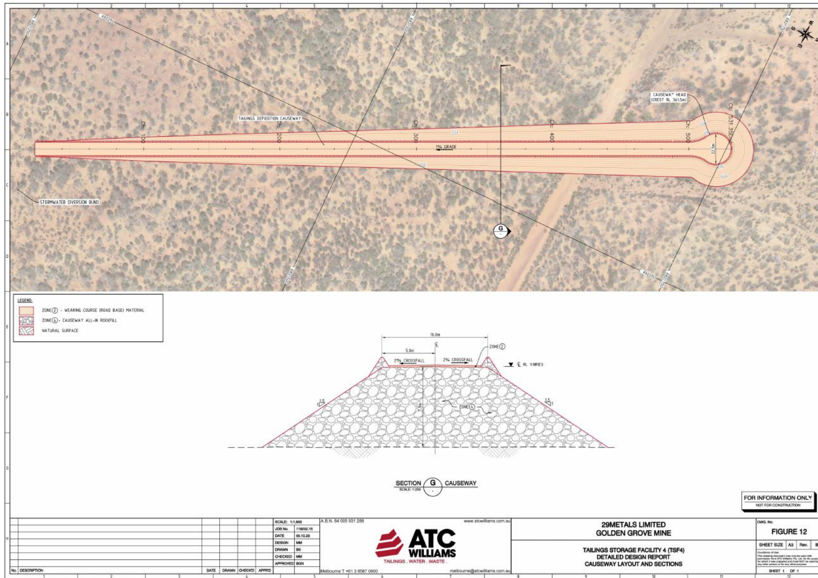
Figure 4: TSF4 causeway
