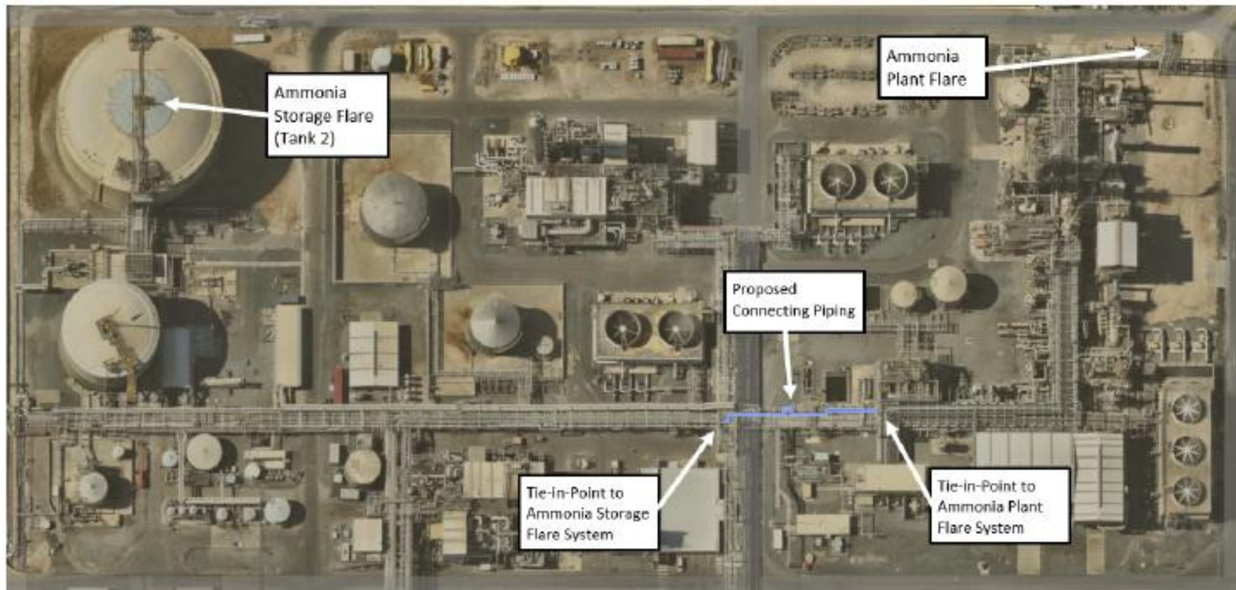
Figure 4: Proposed tie-in for Ammonia Storage and Ammonia Plant flare system
