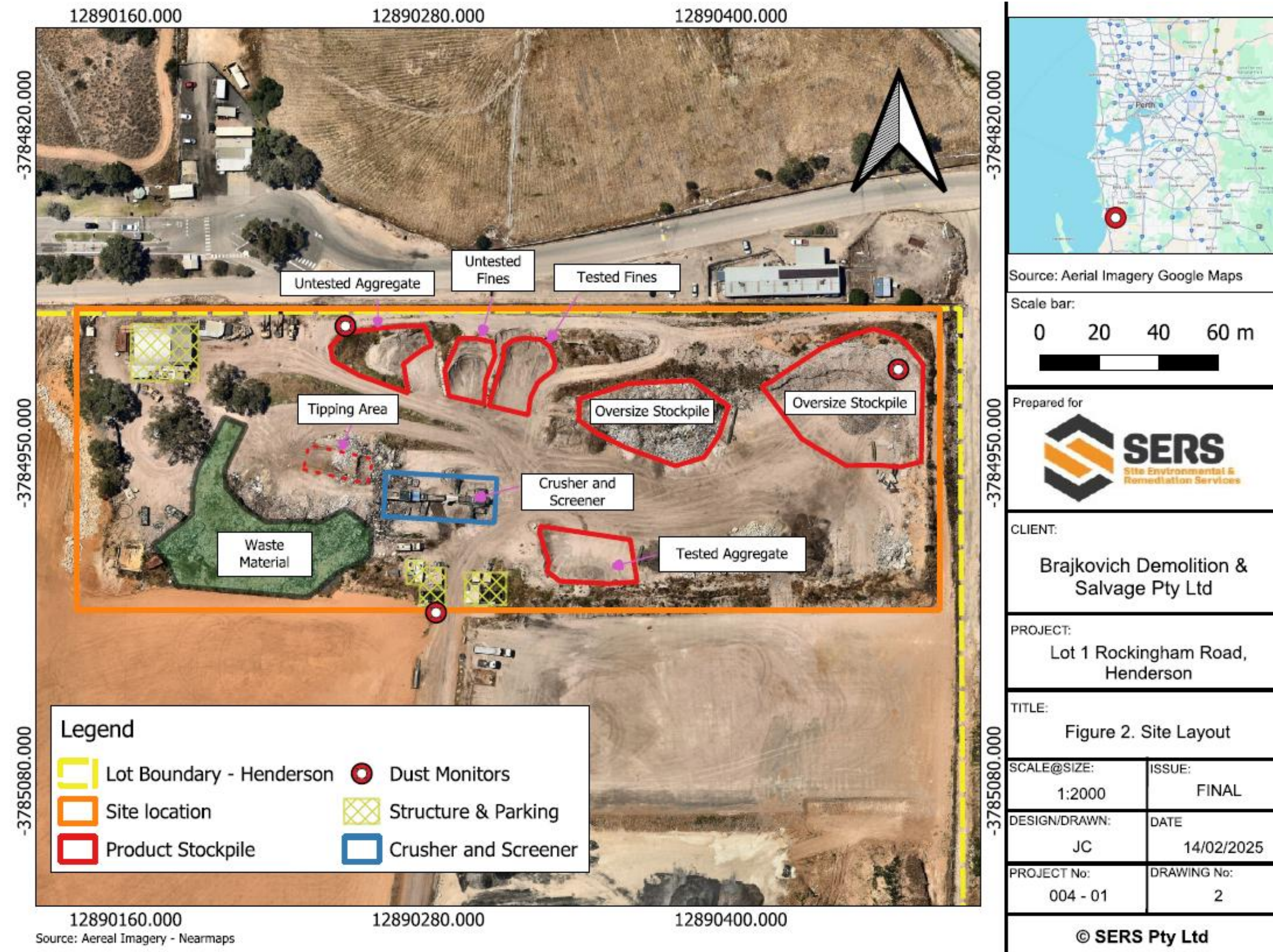
Figure 2: Site layout [source: Dust Management Plan (SERS, 2025)]
