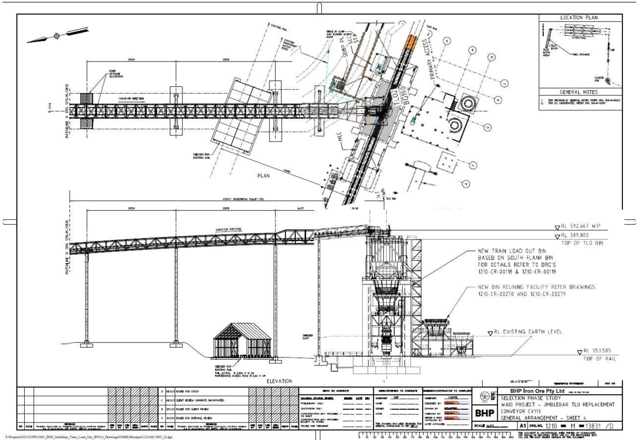
Figure 4: Schematic of the Train Load Out replacement conveyor with dual bins
