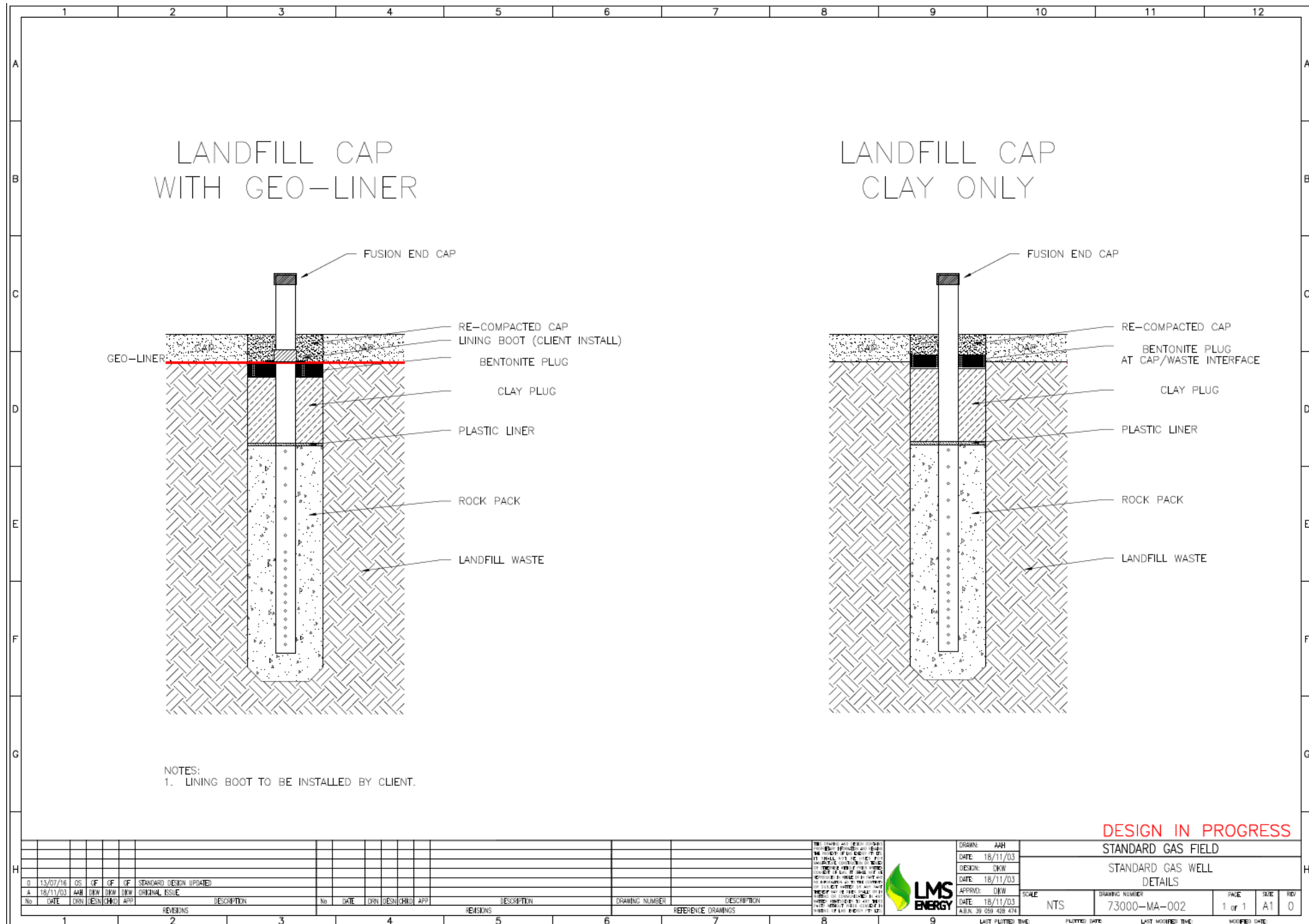
Figure 14: Typical landfill gas well details
