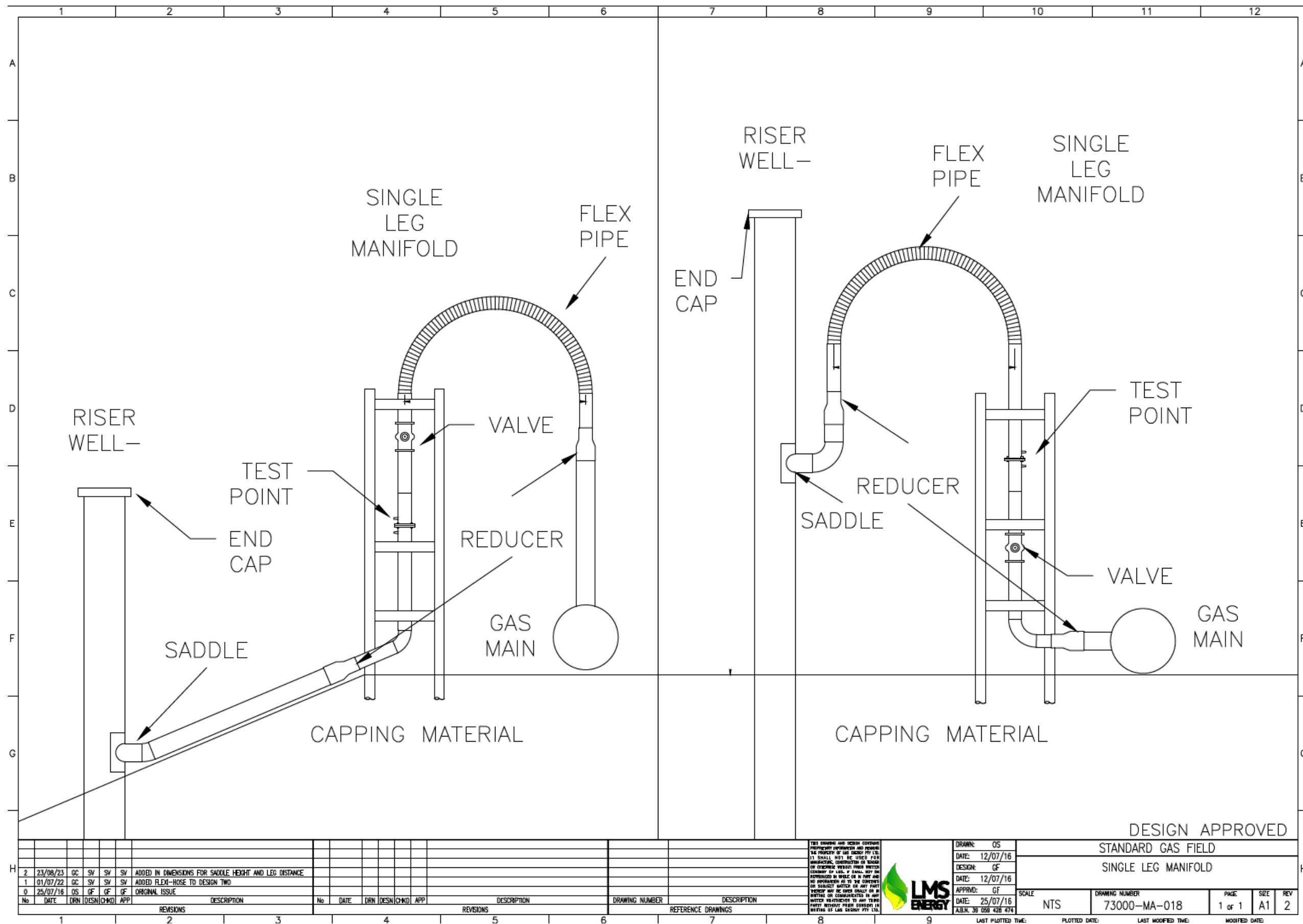
Figure 13: Typical landfill gas manifold design specifications
