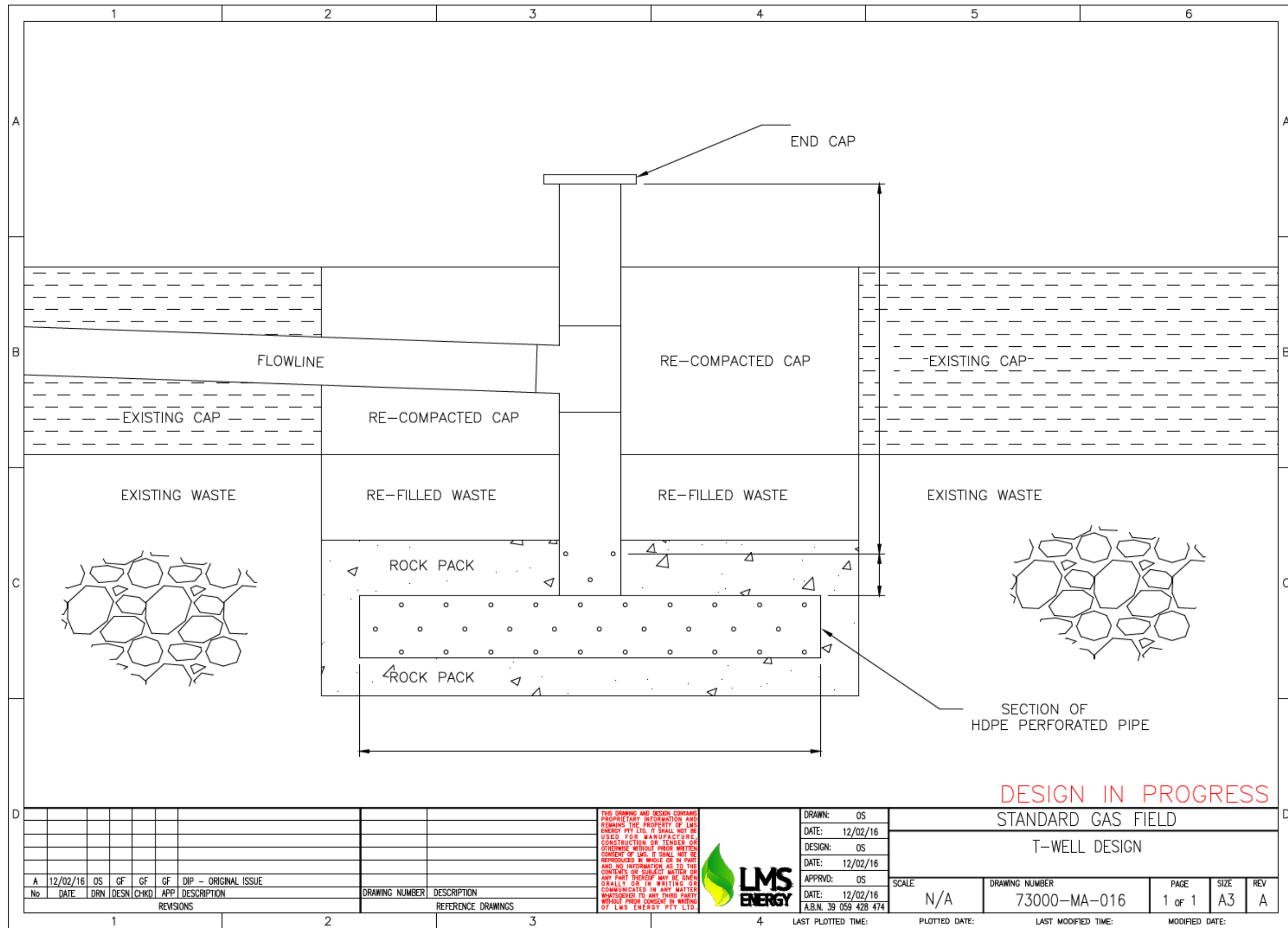
Figure 10: Typical landfill gas t-well design design specifications
