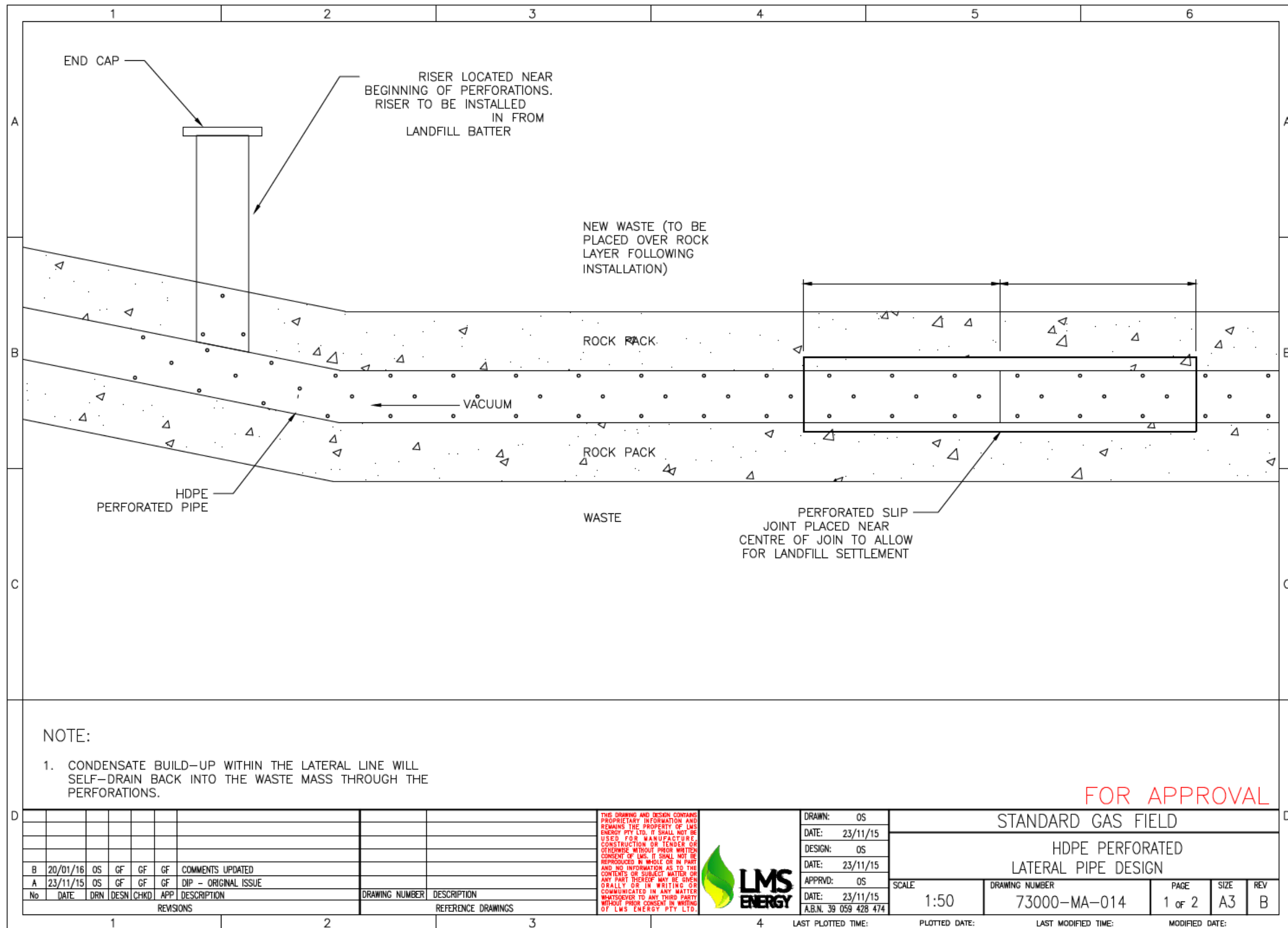
Figure 9: Typical landfill gas HDPE perforated lateral pipe design specification
