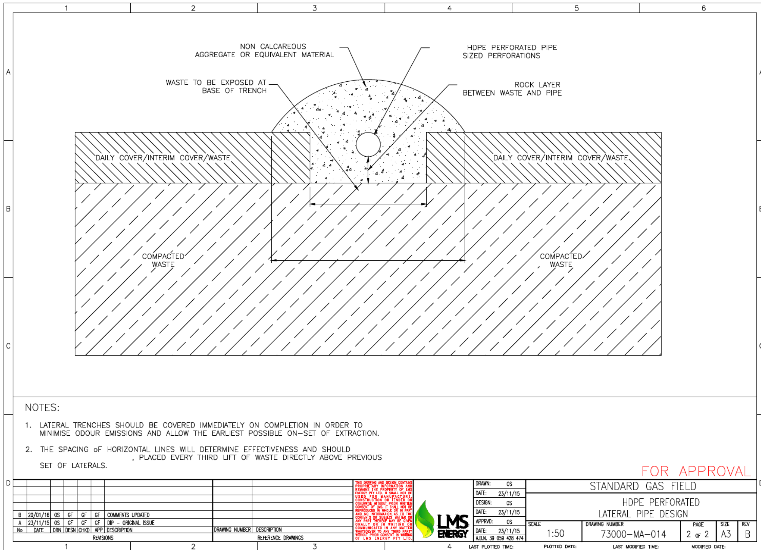
Figure 15: Typical landfill gas HDPE perforated lateral pipe design specifications
