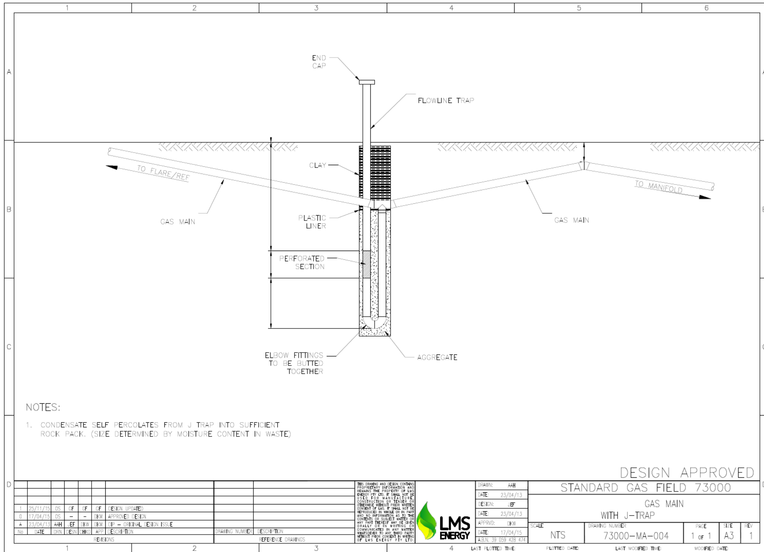
Figure 11: Typical landfill gas main with j-trap design specifications
