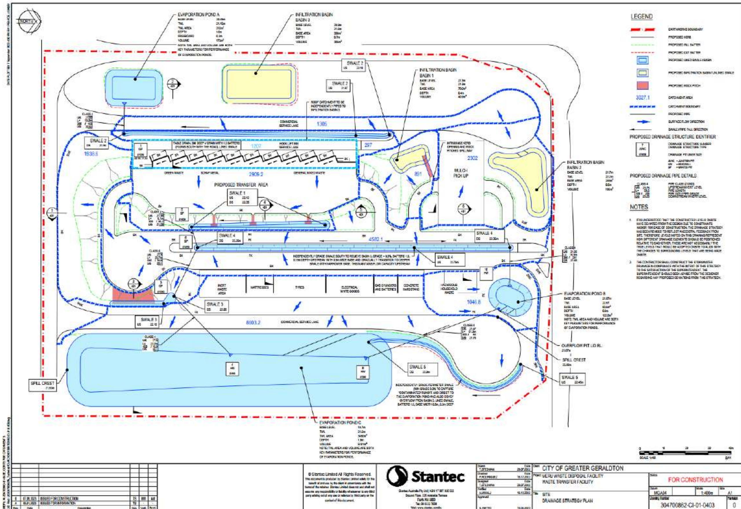
Figure 7: Community Waste Transfer Station Layout Plan
