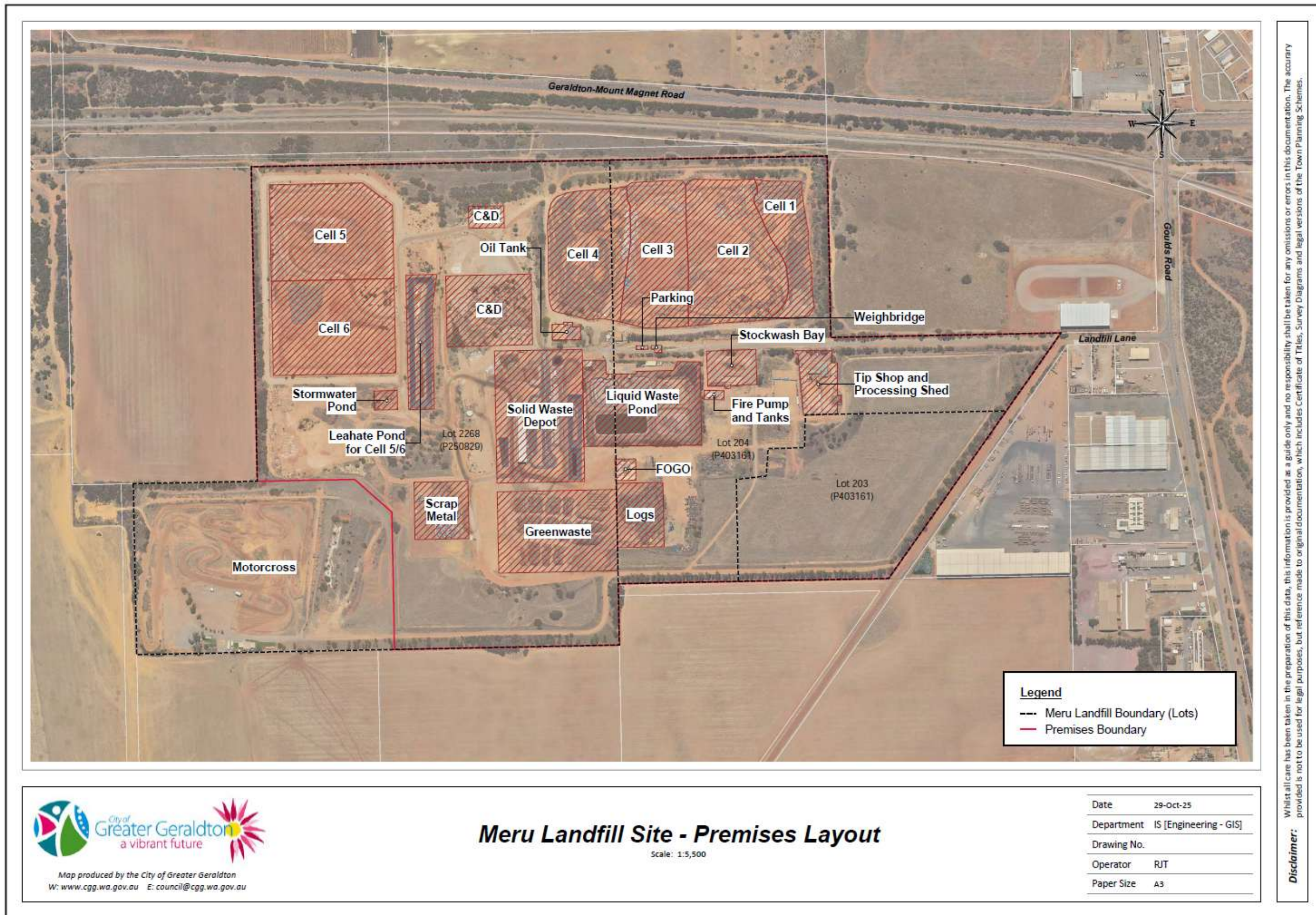
Figure 4: Premises layout
