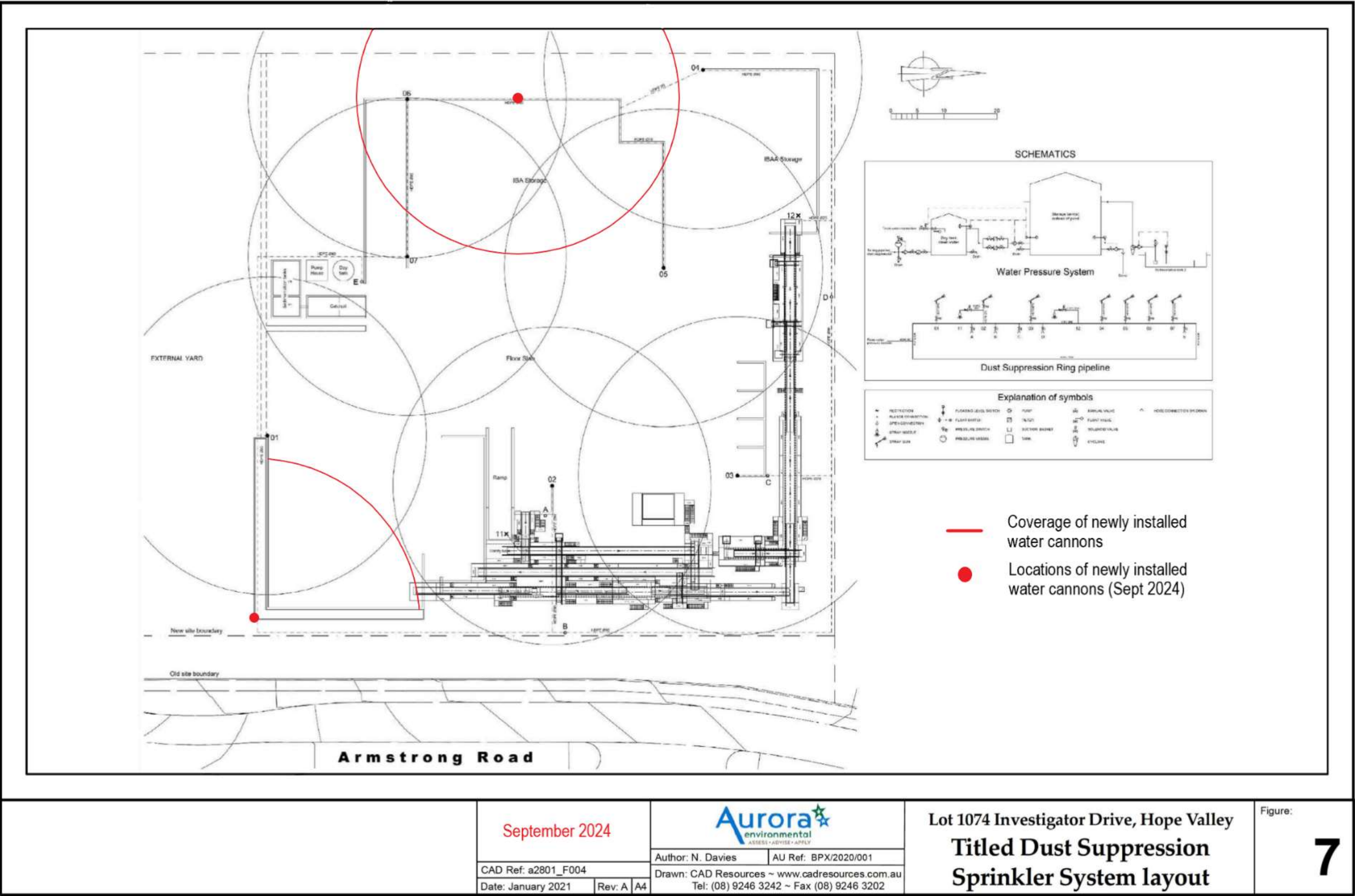
Figure 3: Premises dust suppression system/sprinkler layout.
