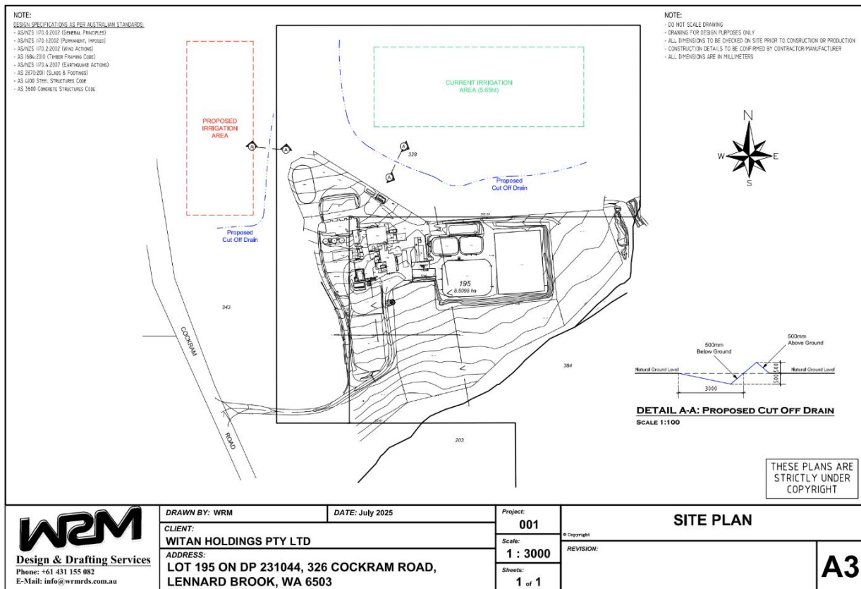
Figure 5: Proposed cut off drain location and desing.
