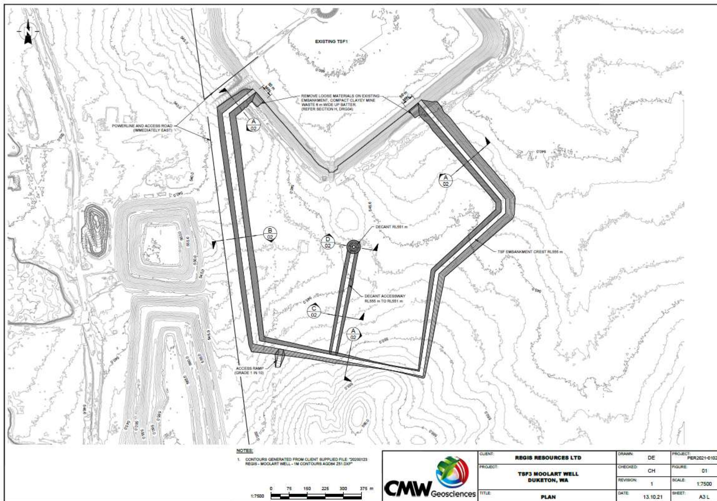
Figure 2 – Moolart Well TSF3 general arrangements
