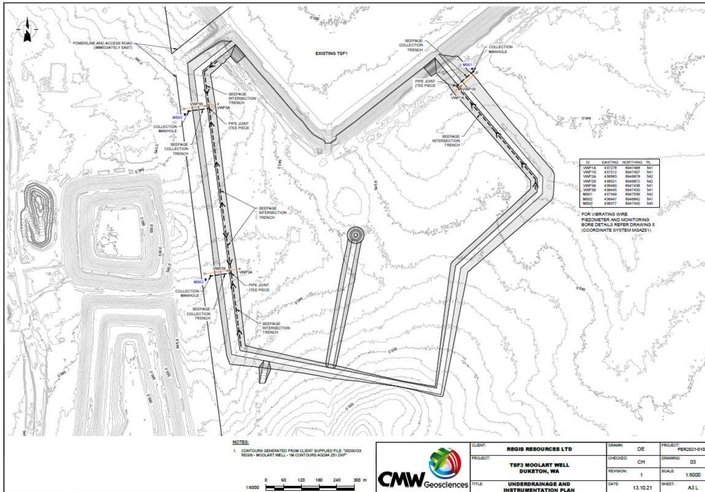
Figure 5 – Moolart Well TSF3 – Underdrainage and instrumentation plan.
