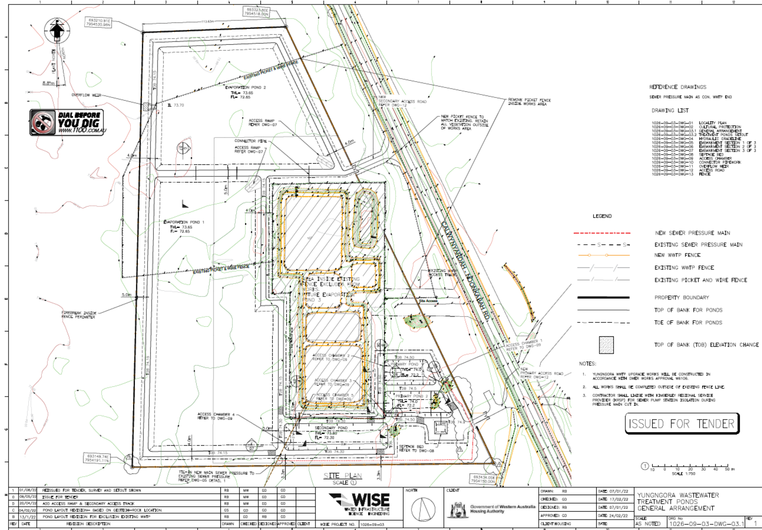
Figure 2: Layout and general arrangement of the works
