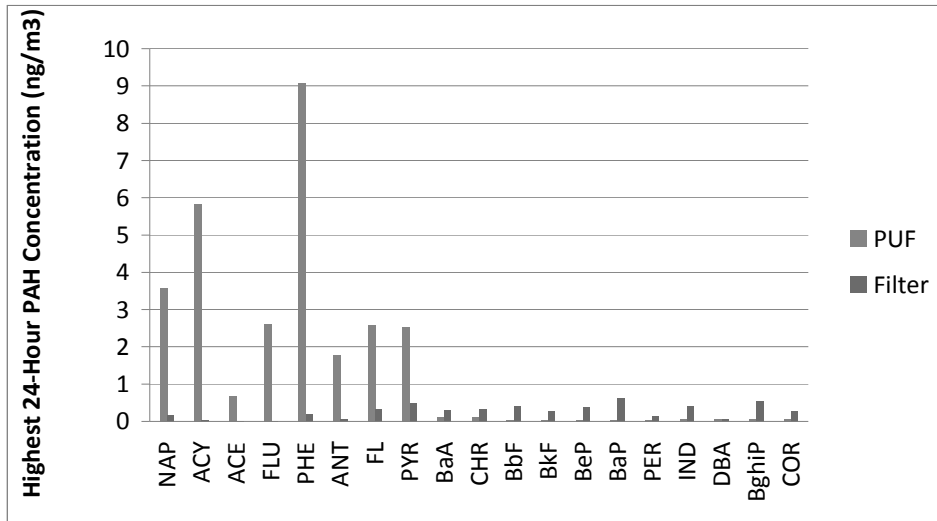
Figure 14. Highest 24-hour concentrations (ng/m 3 ) for each PAH captured on the PUF and filter portions of the air sample.
