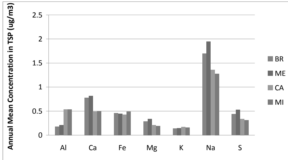
Figure 10. Annual mean concentrations (µg/m³) for selected chemical species in TSP at Melville (ME ), Brentwood (BR), Caversham (CA) and Midvale Primary School (MI).
