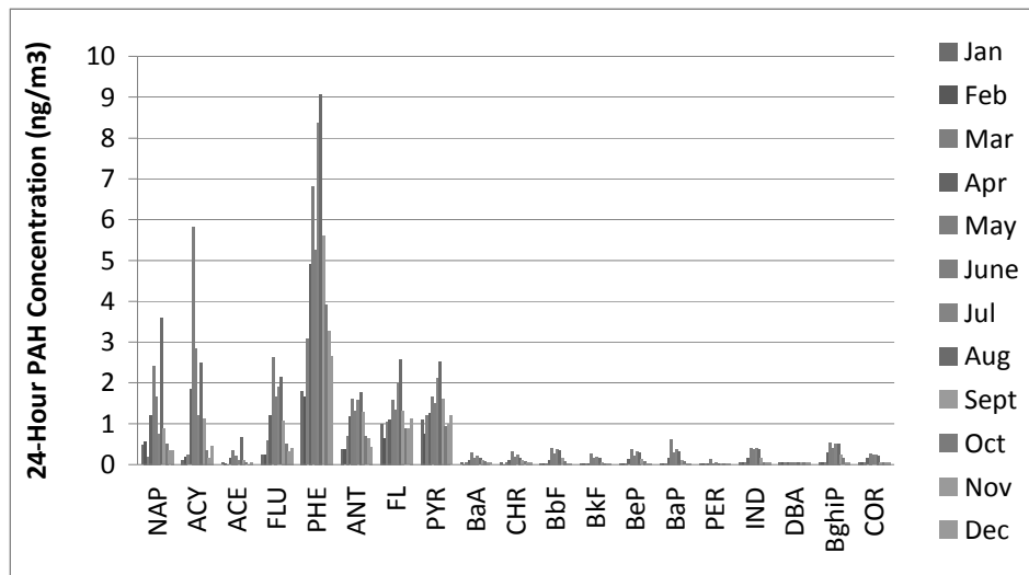
Figure 17. The highest 24-hour concentrations (ng/m 3 ) by month for each PAH captured on the PUF and filter portions of the air sample.
