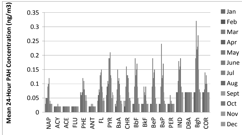
Figure 16. The mean concentrations (ng/m 3 ) by month for each PAH captured on the filter portion of the air sample.
