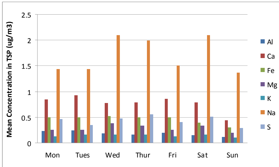
Figure 9a. Mean concentrations (µg/m³) by day-of-week for selected chemical species in TSP at Brentwood (BR).
