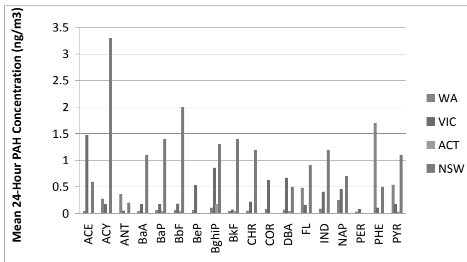
Figure 22. Average 24-hour concentrations for ambient PAHs measured in Australia
