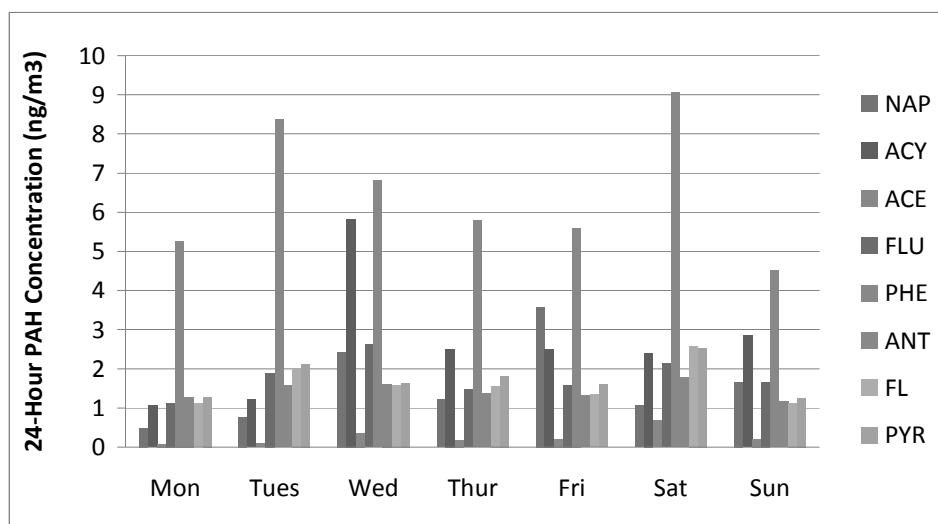
Figure 20. The highest 24-hour concentrations ( \text{ng}/\text{m}^3 ) by day-of-week for selected PAHs captured on the PUF portion of the air sample.
