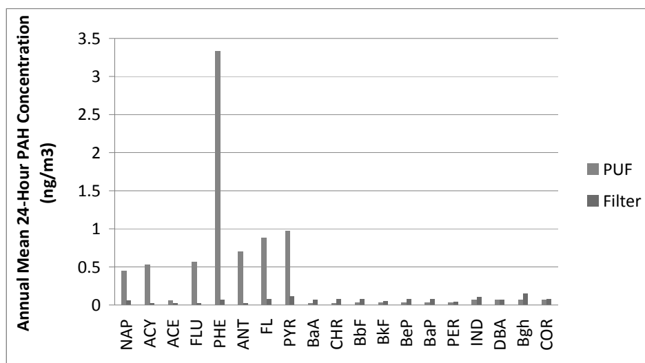
Figure 13. Annual mean concentrations ( \text{ng}/\text{m}^3 ) for each PAH captured on the PUF and filter portions of the air sample.
