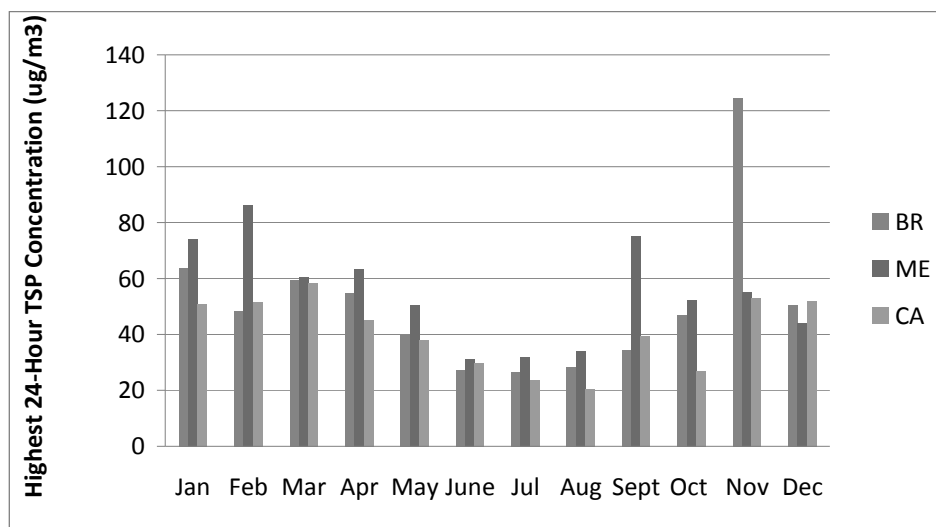
Figure 6. Highest 24-hour TSP concentrations ( \mu\text{g}/\text{m}^3 ) for each month at Caversham (CA), Melville (ME) and Brentwood (BR).
