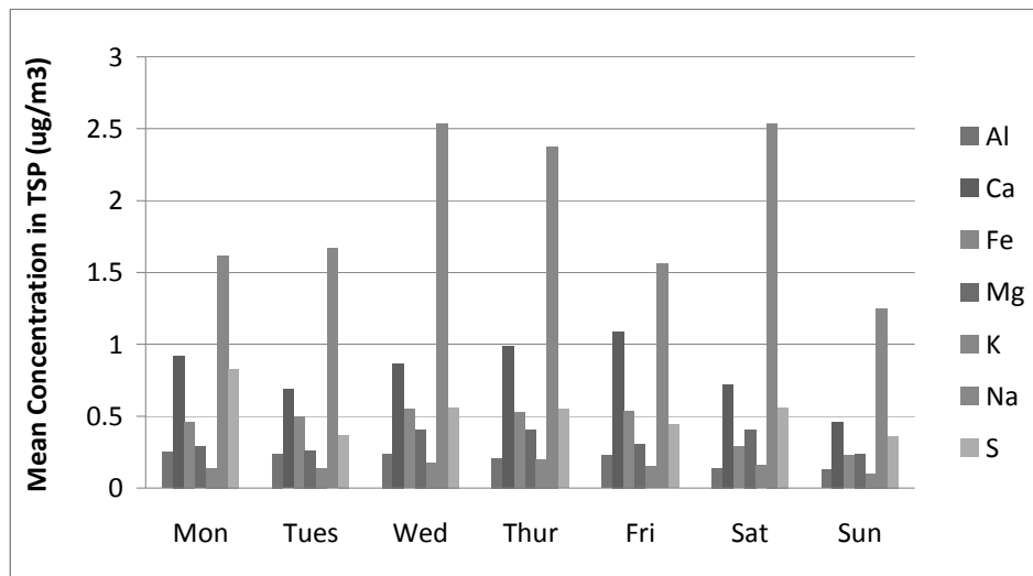
Figure 9b. Mean concentrations (µg/m³) by day-of-week for selected chemical species in TSP at Melville (ME).
