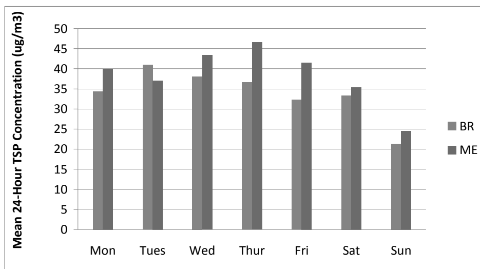
Figure 3. Mean 24-hour TSP concentrations ( \mu\text{g}/\text{m}^3 ) by day-of-the-week at Brentwood (BR) and Melville (ME).
