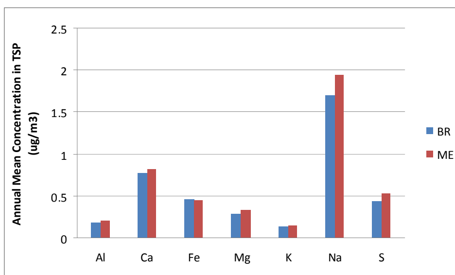
Figure 7. Annual mean concentrations ( \mu\text{g}/\text{m}^3 ) for selected chemical species in TSP at Melville (ME) and Brentwood (BR).
