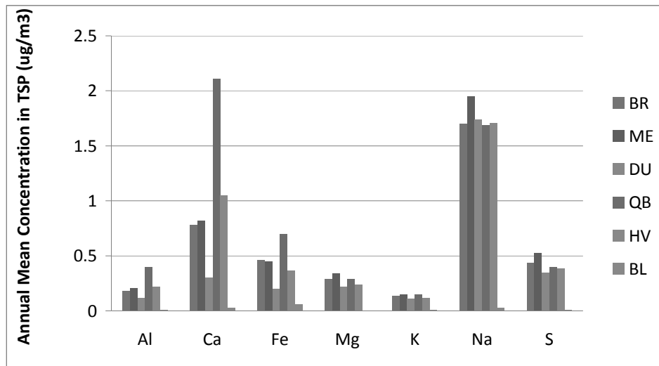
Figure 11. Annual mean concentrations (µg/m³) for selected chemical species in TSP at Melville (ME ), Brentwood (BR), Duncraig (DU), Queens Buildings (QB), Hope Valley (HV) and Bibra Lake (BL).
