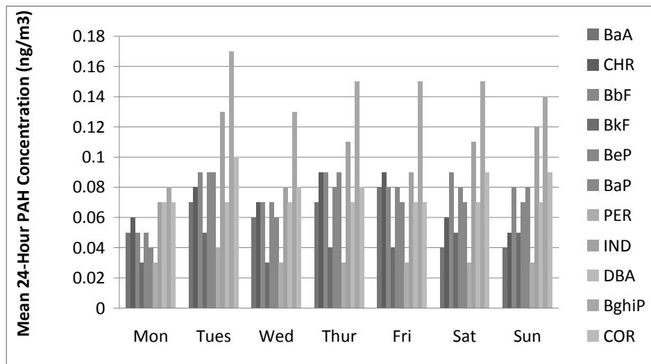
Figure 19. The mean concentrations (ng/m 3 ) by day-of-week for selected PAHs captured on the filter portion of the air sample.
