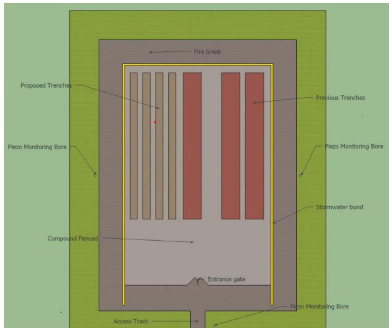
Figure 1: Site layout
