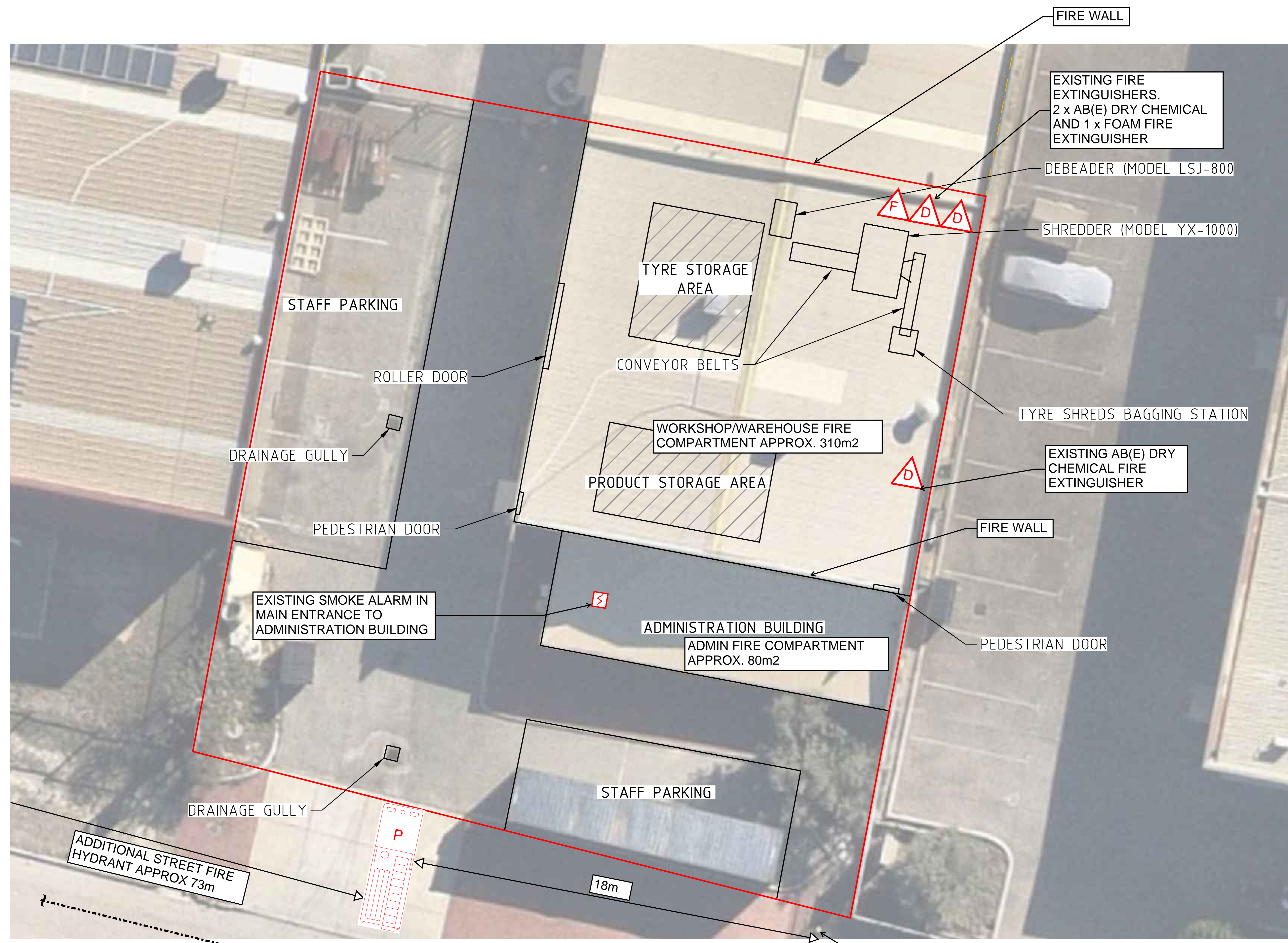
1 PLAN - BUILDING LAYOUT
