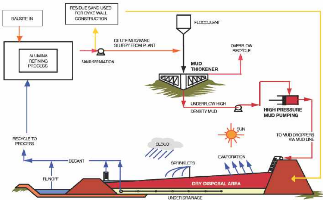
Figure 4-1: Dry stacking process used at Alcoa's residue area.
