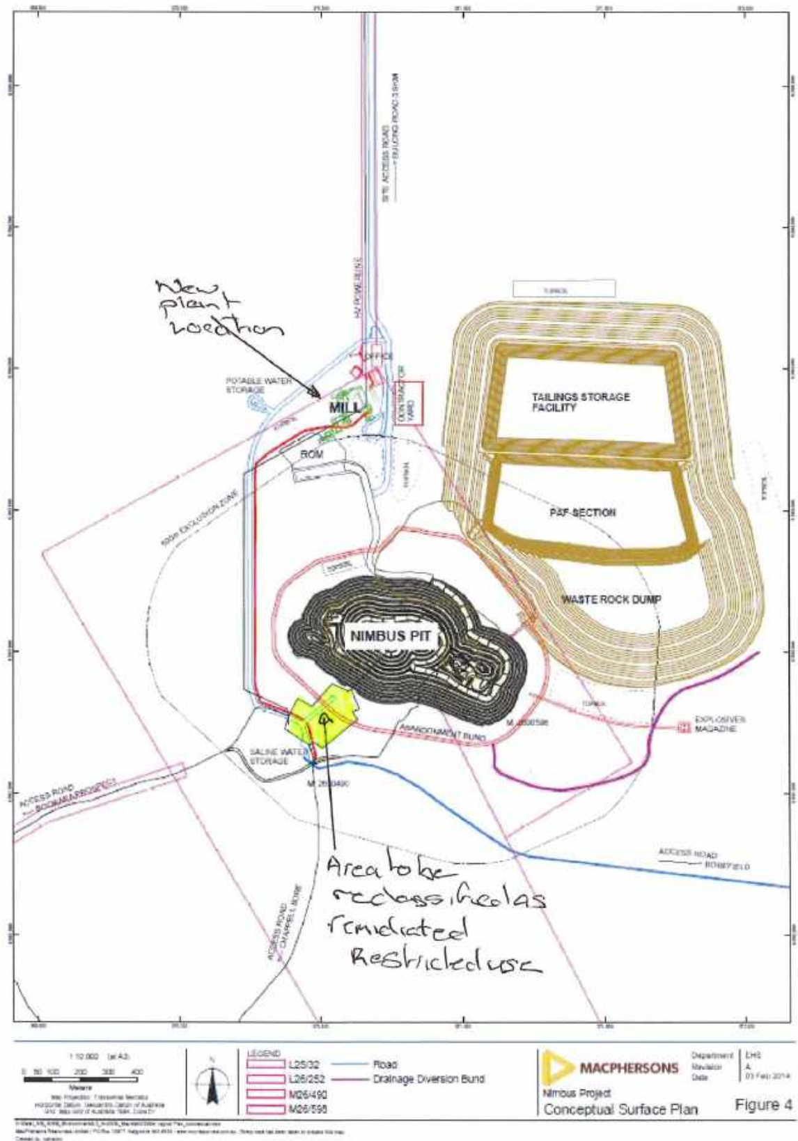
Figure 4: Conceptual Surface Plan
