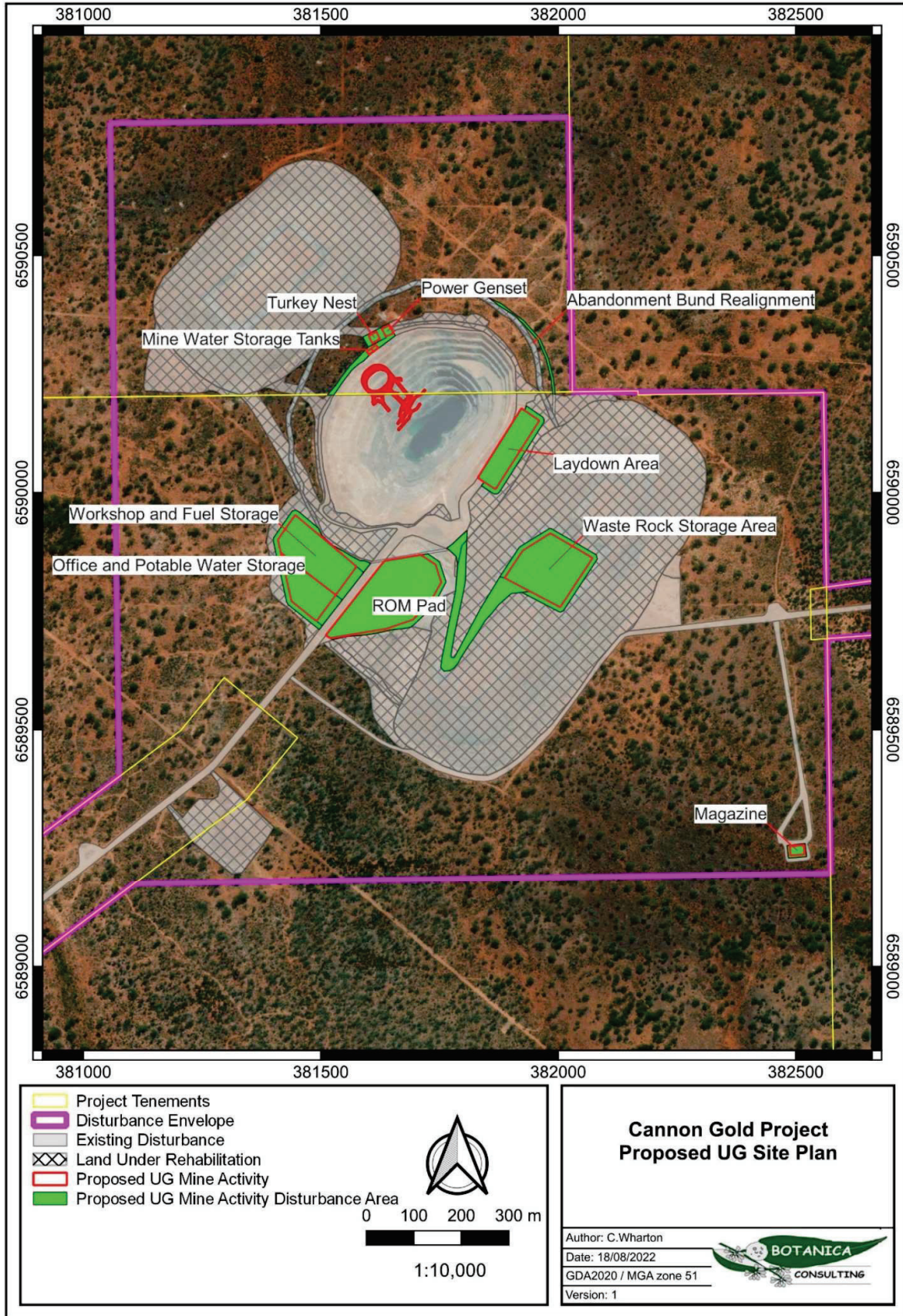
Figure 4-10: Proposed Underground Site Plan
