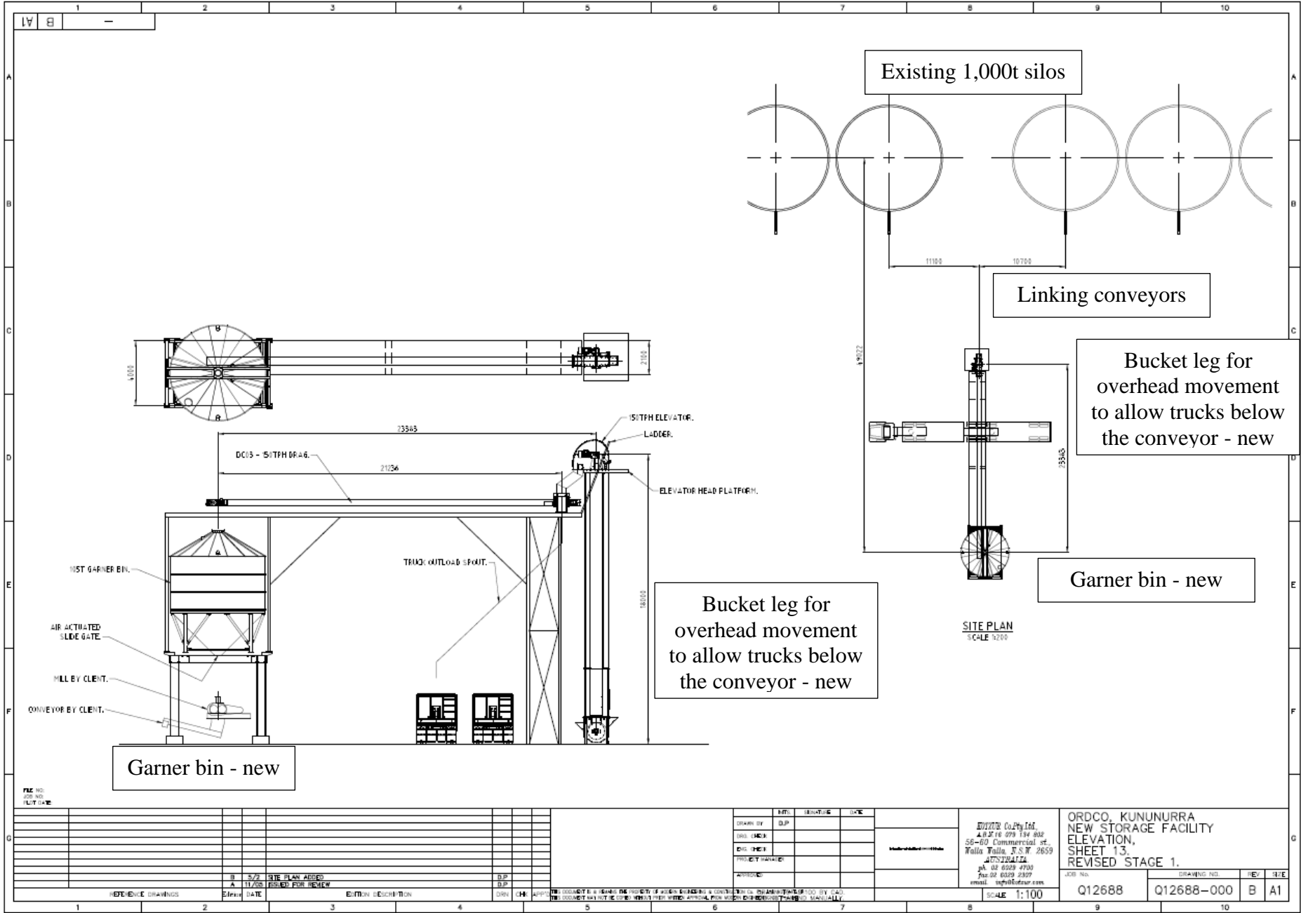
Attachment 3b – Construction diagram
