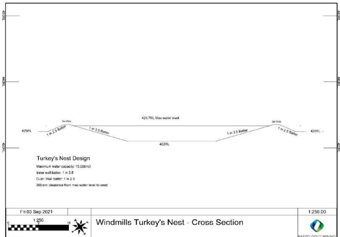
Figure 24: Cross section of Windmills Turkey's Nest
