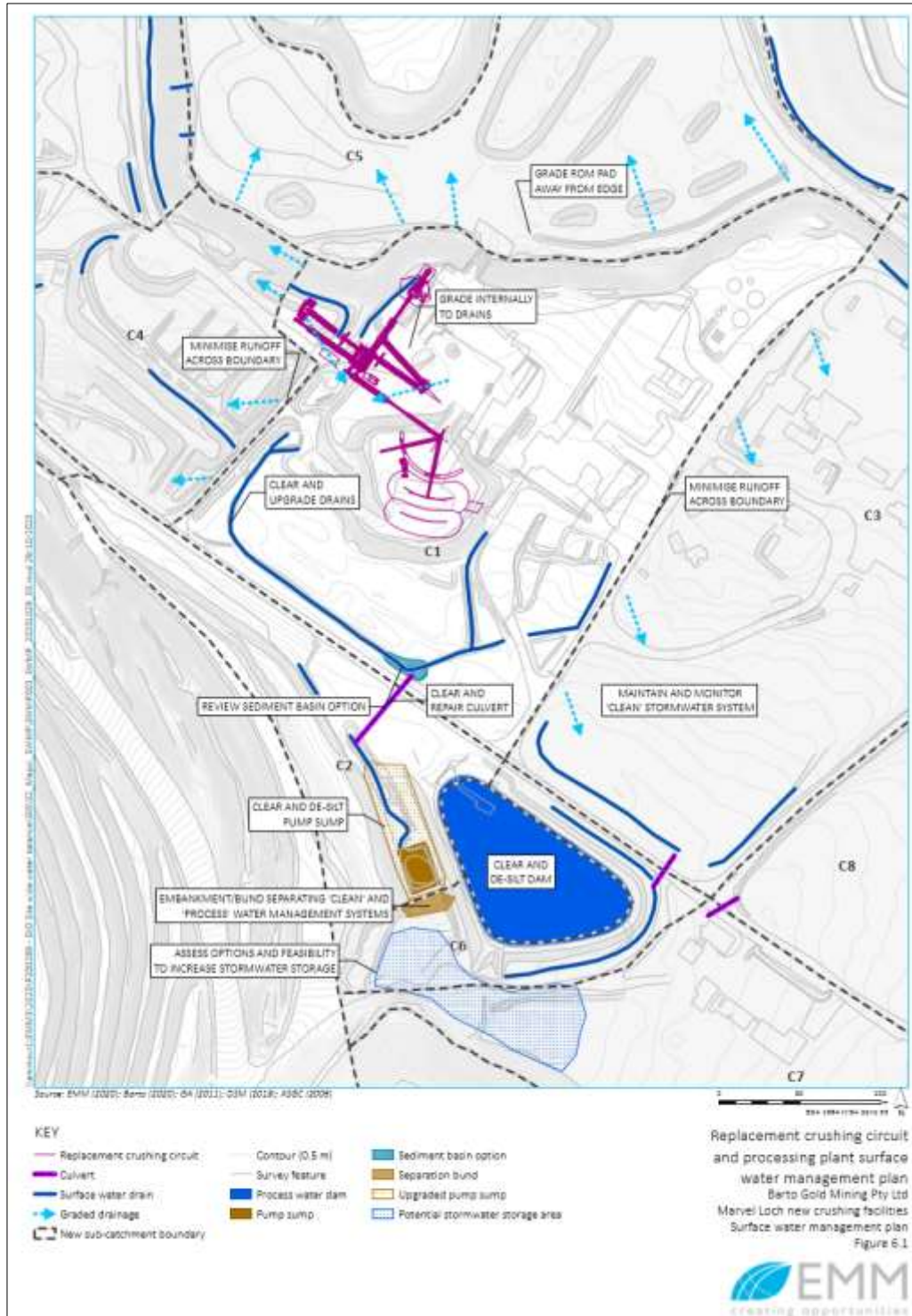
Figure 22: Map of stormwater infrastructure to be constructed in accordance with condition 24 Table 6.
