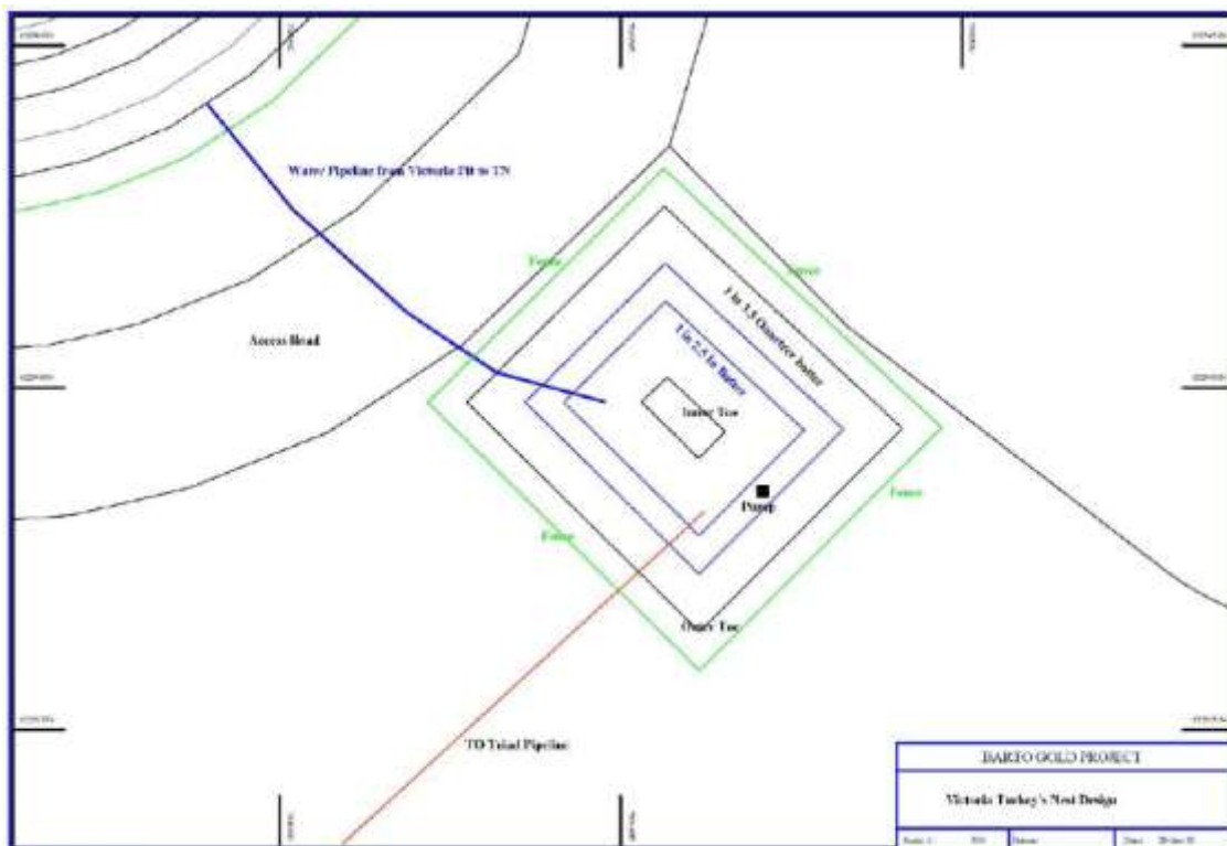
Figure 25: Layout map of the Victoria's Turkey's Nest and dewatering pipeline from Victoria's Pit
