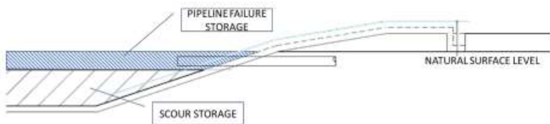
Figure 27: Diagrammatic representation of scour sump to be created for the section of the Axehandle Pipeline that will sit above the ground
