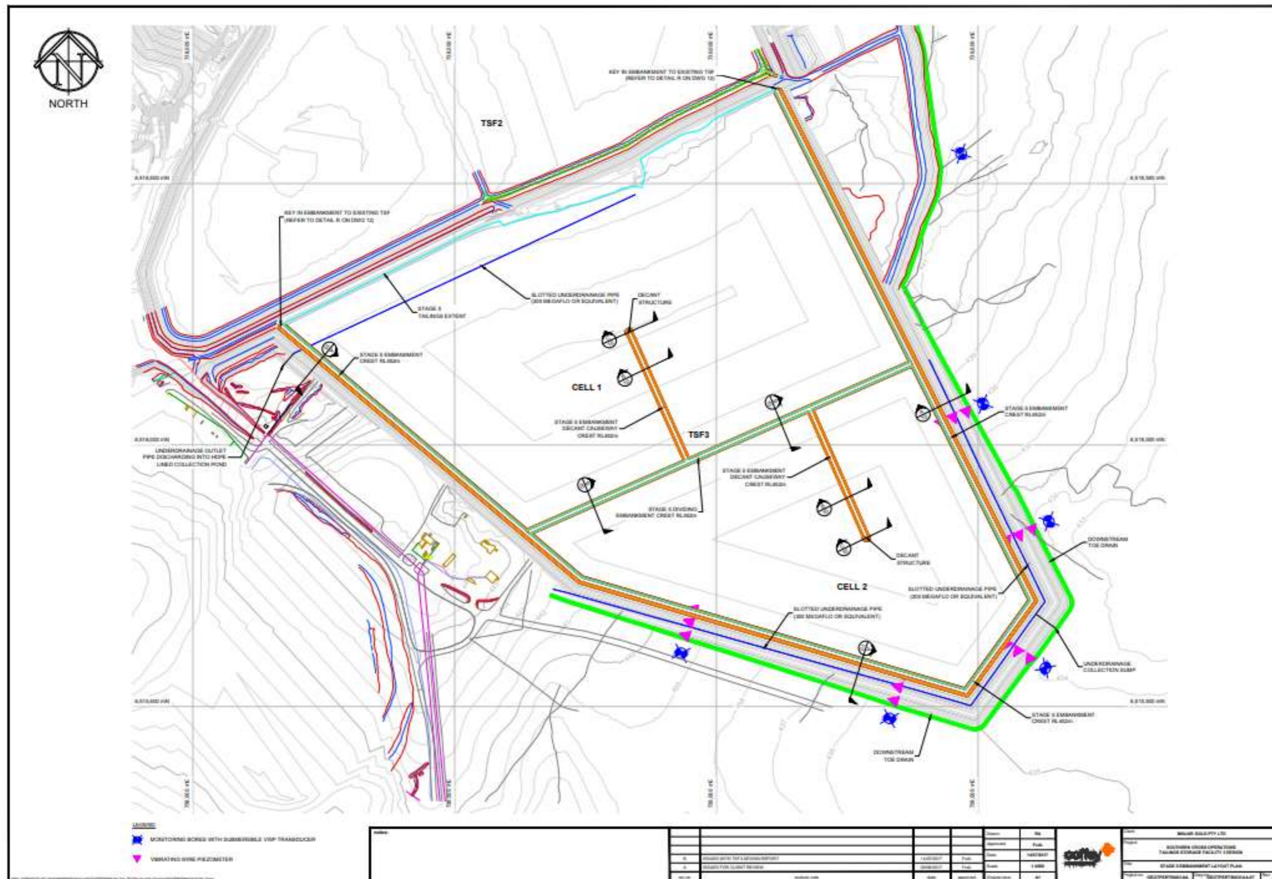
Figure 30: TSF3 Stage 5 Embankment Layout plan
