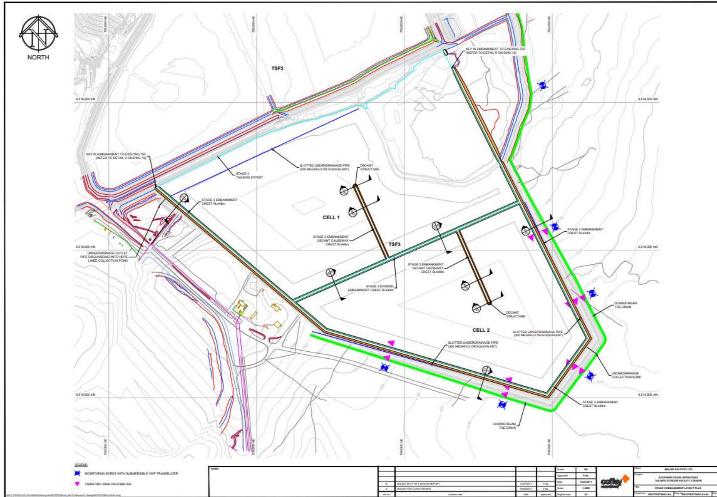
Figure 28: TSF 3 Stage 3 Embankment Layout plan
