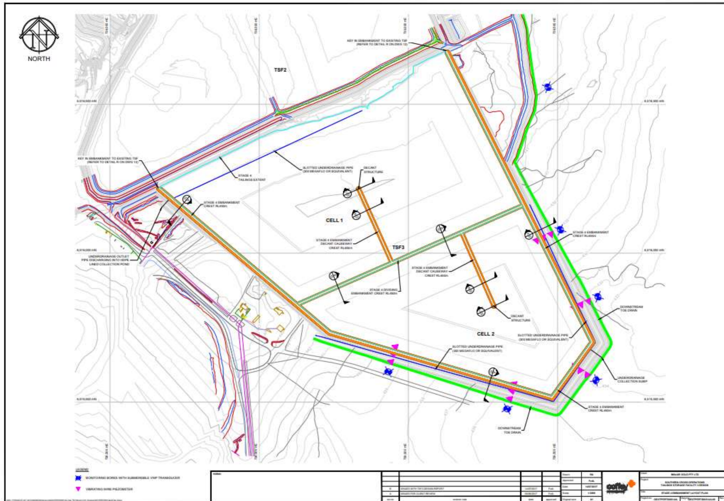
Figure 29: TSF3 Stage 4 Embankment Layout plan
