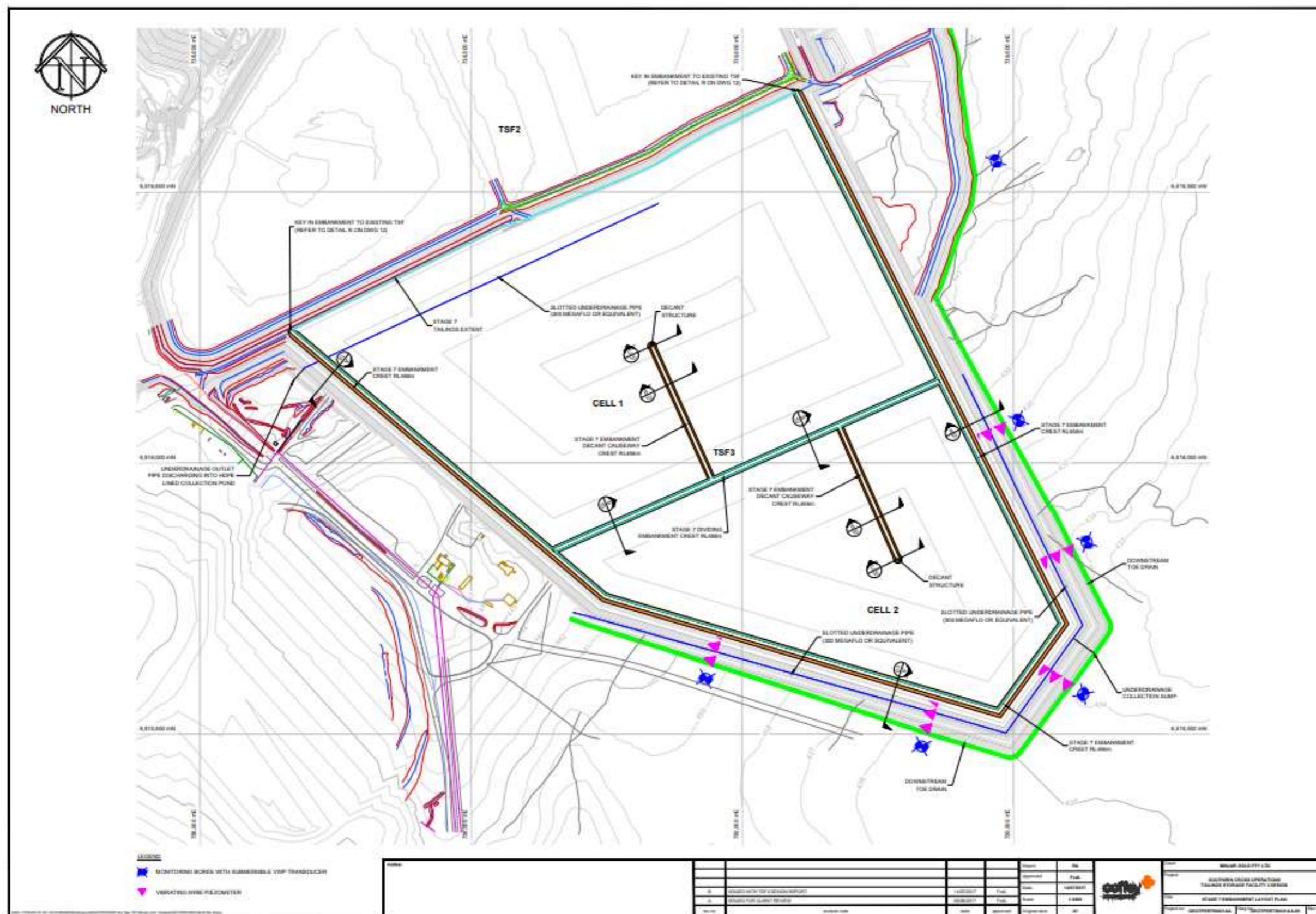
Figure 32: TSF3 Stage 7 Embankment Layout plan
