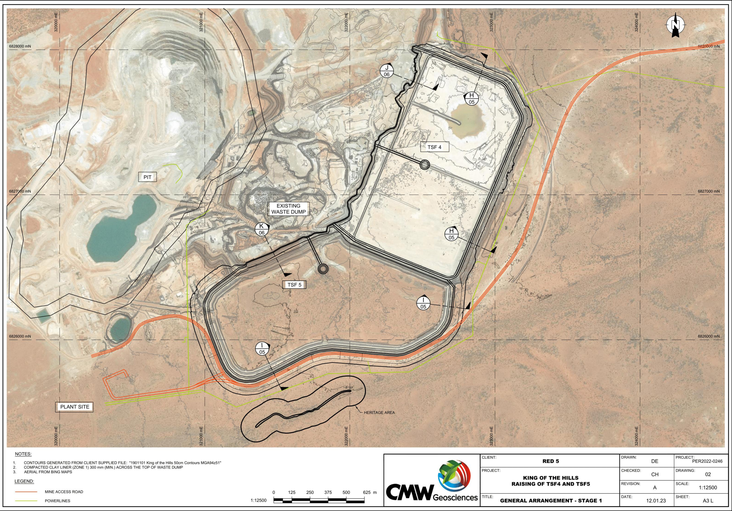
Figure 2: TSF4 site layout (Stage 7 expansion and embankment raise)
