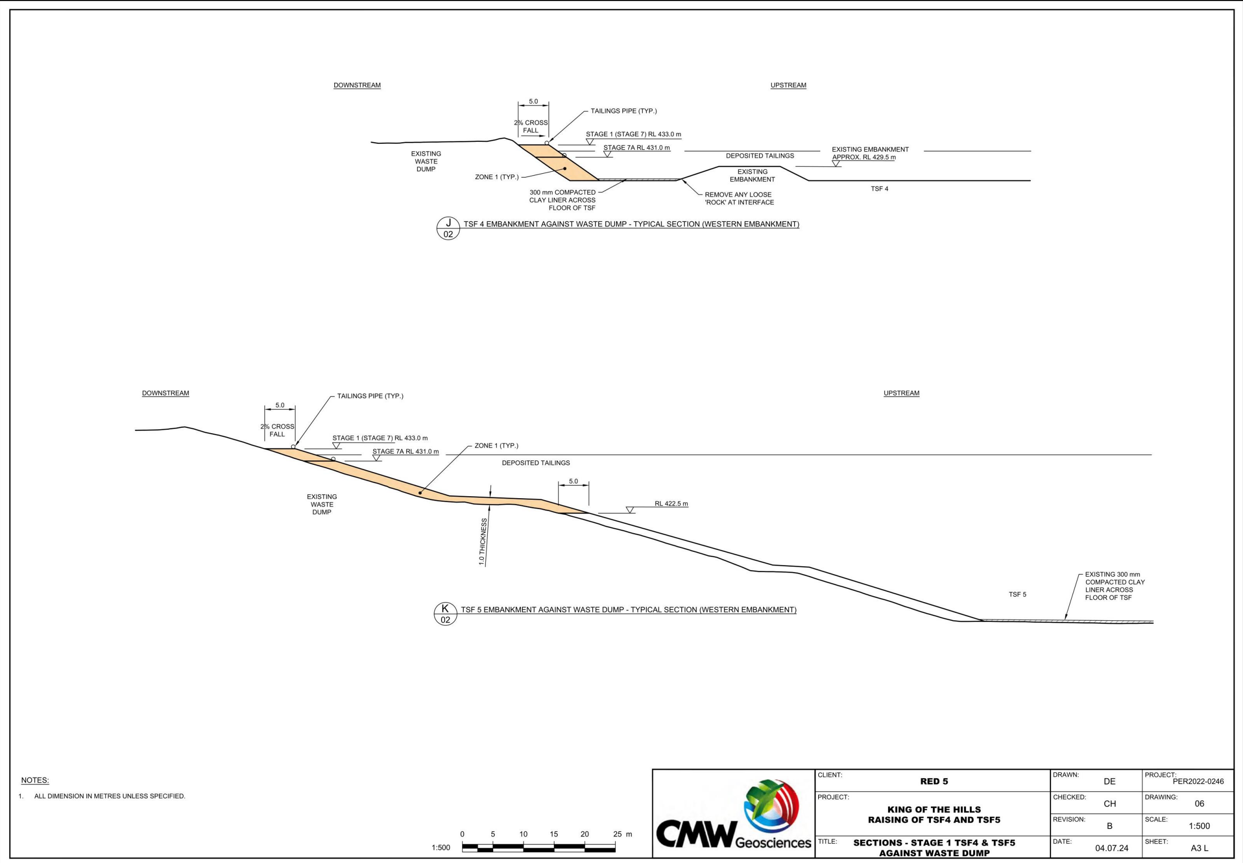
Figure 8: Design drawing for TSF4 Stage 1 embankment (western embankment)
