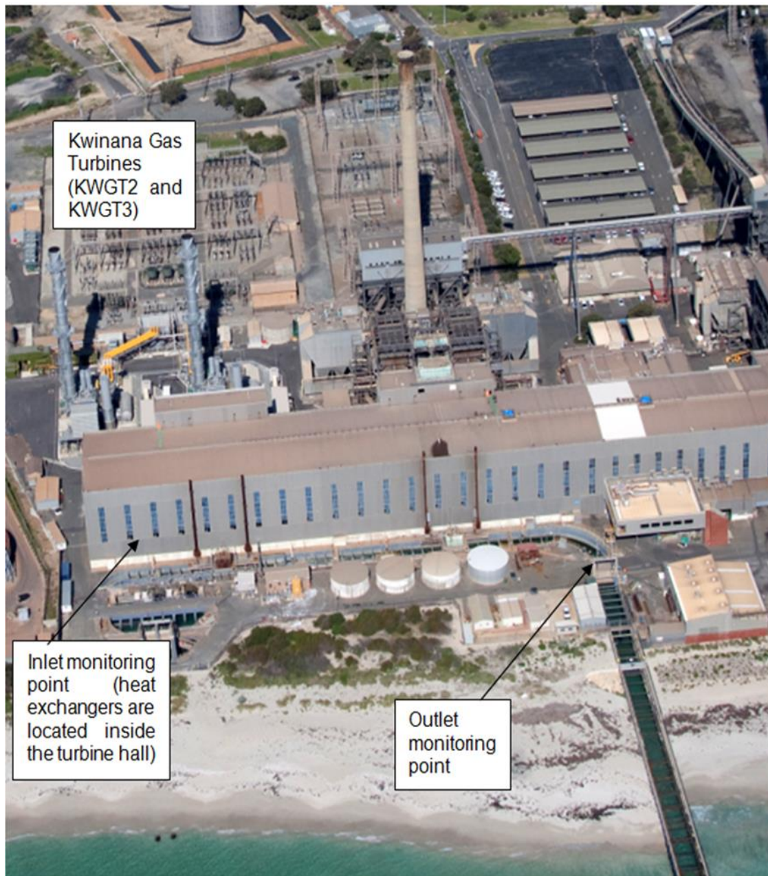
Figure 2: Water discharge points
