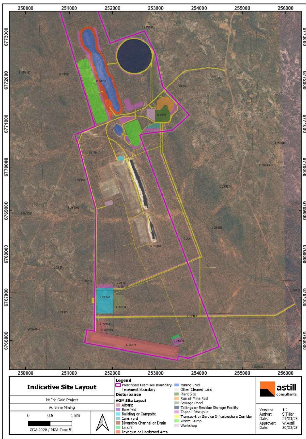
Figure 2: Site Layout
