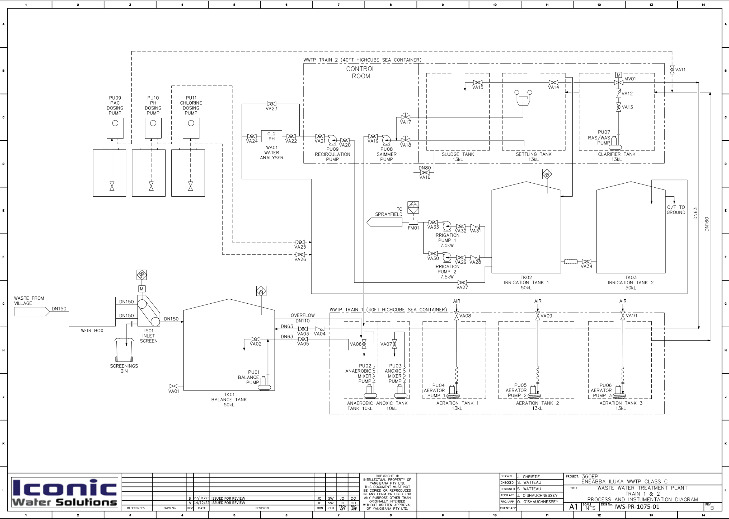
Figure 3: Wastewater treatment plant process design
