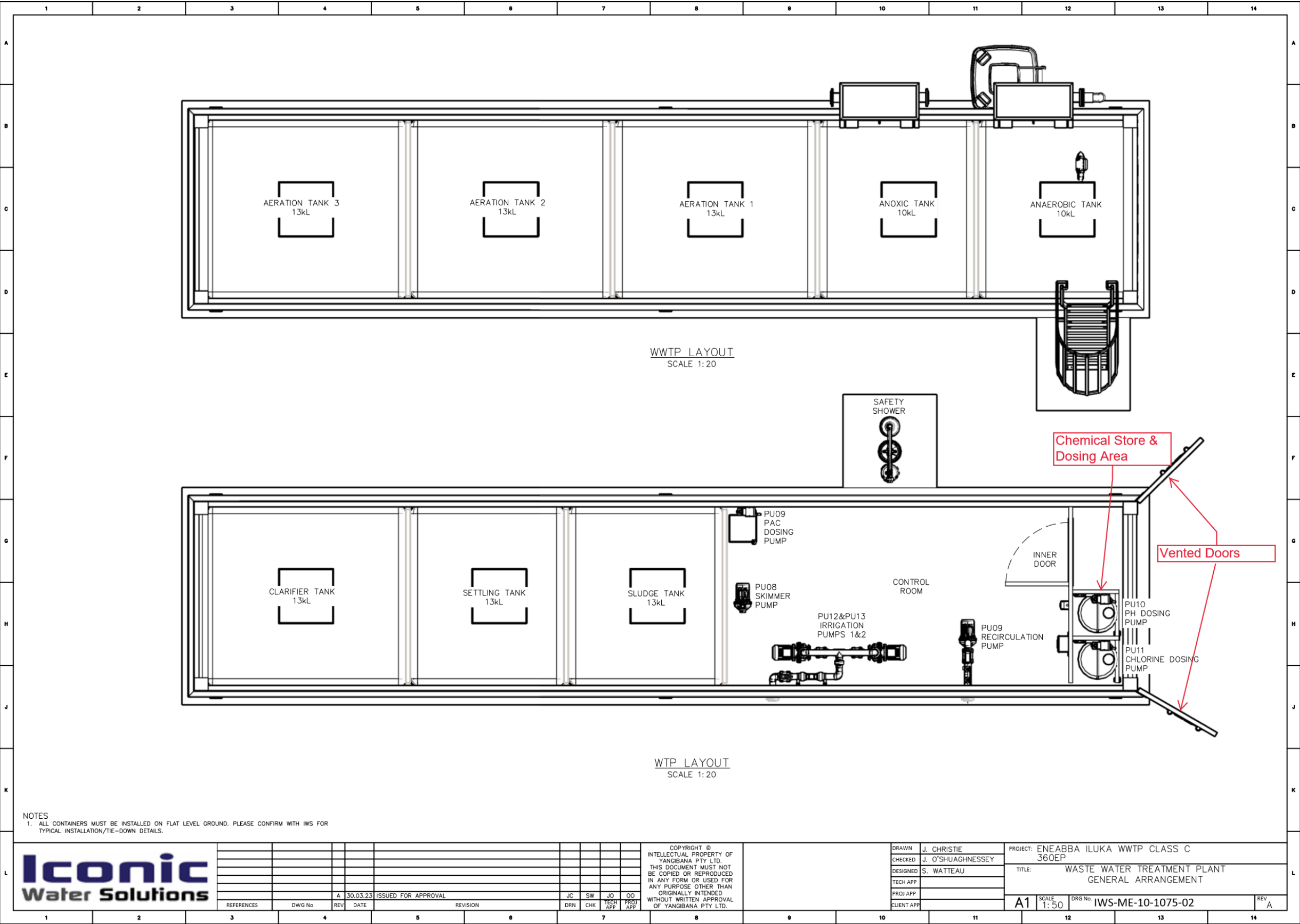
Figure 5: Treatment unit arrangement
