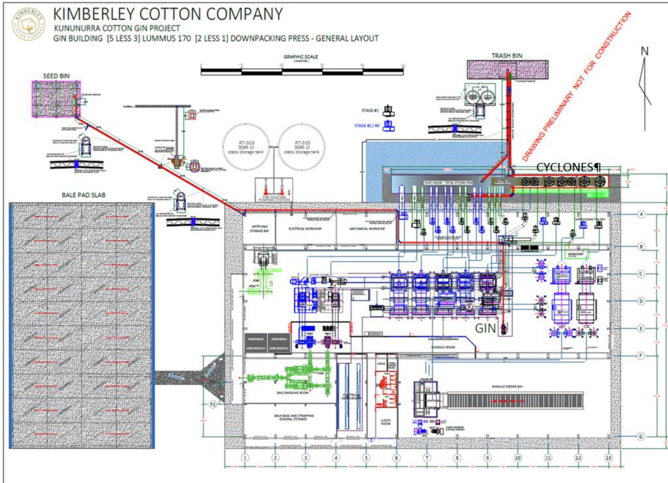
Figure 2: Map of the layout within the gin building for stages 1 and 2 within the prescribed premises
