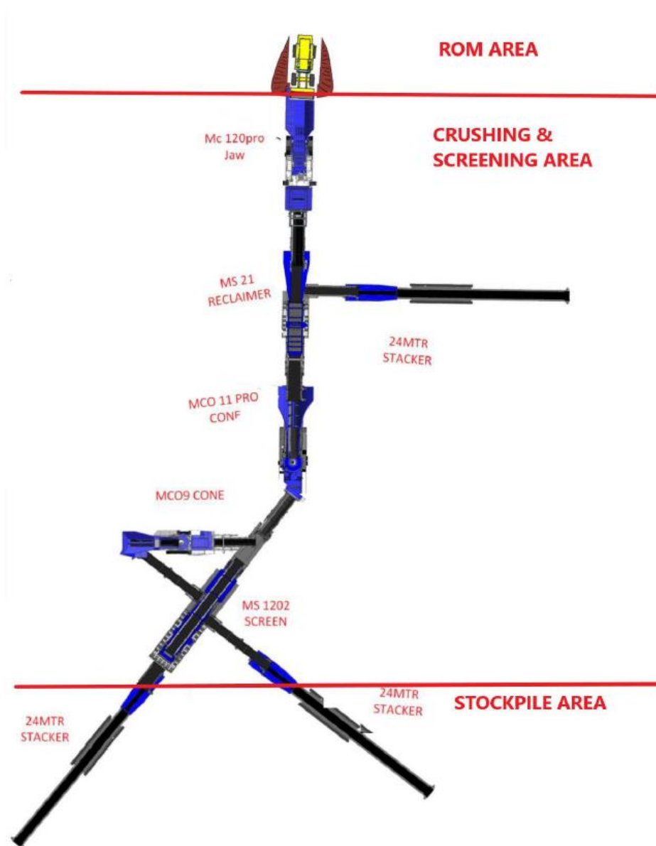
Figure 2: Indicative site layout for screening and crushing plant
