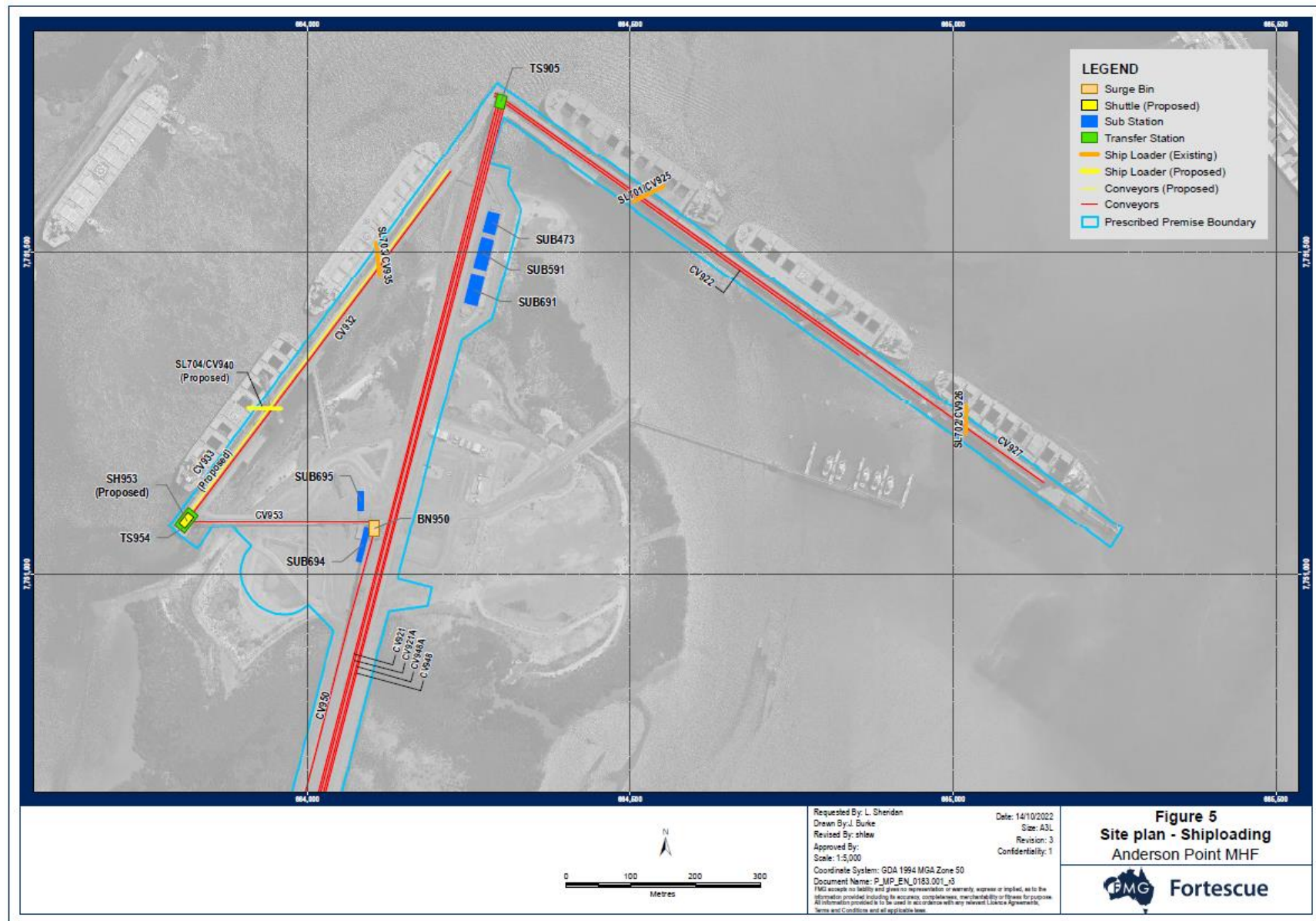
Figure 5: Site plan – shiploading
