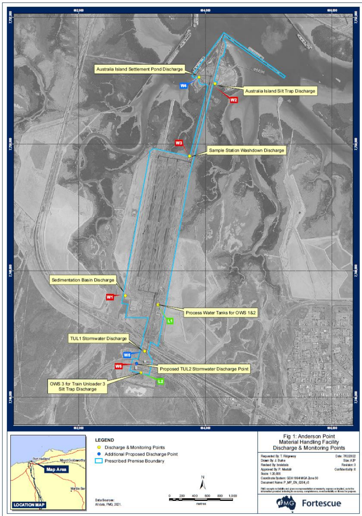
Figure 9: Stormwater and washwater discharges
