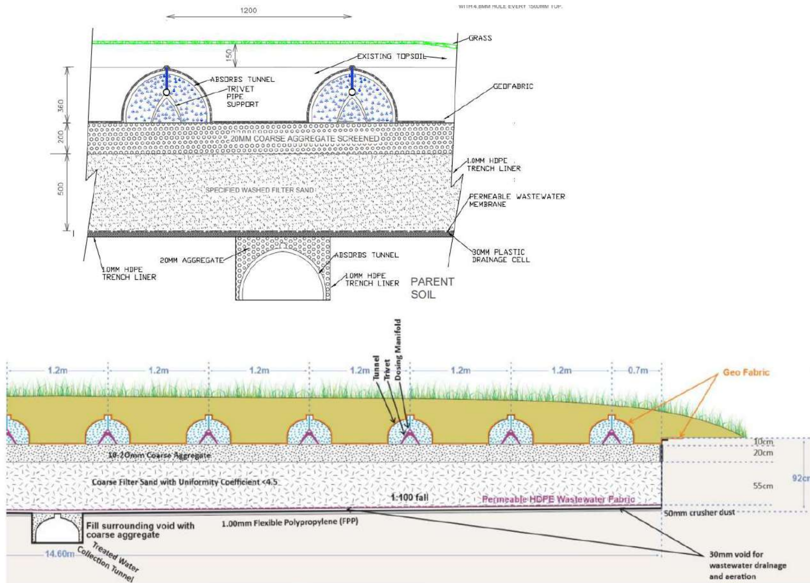
Figure 8: Cross section layout of secondary wastewater treatment filter beds (ABSORB beds depicted in Figure 7)
