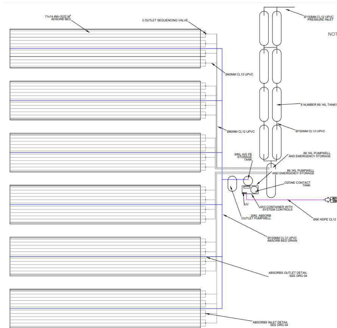
Figure 7: Design layout of Passive WWTP infrastructure
