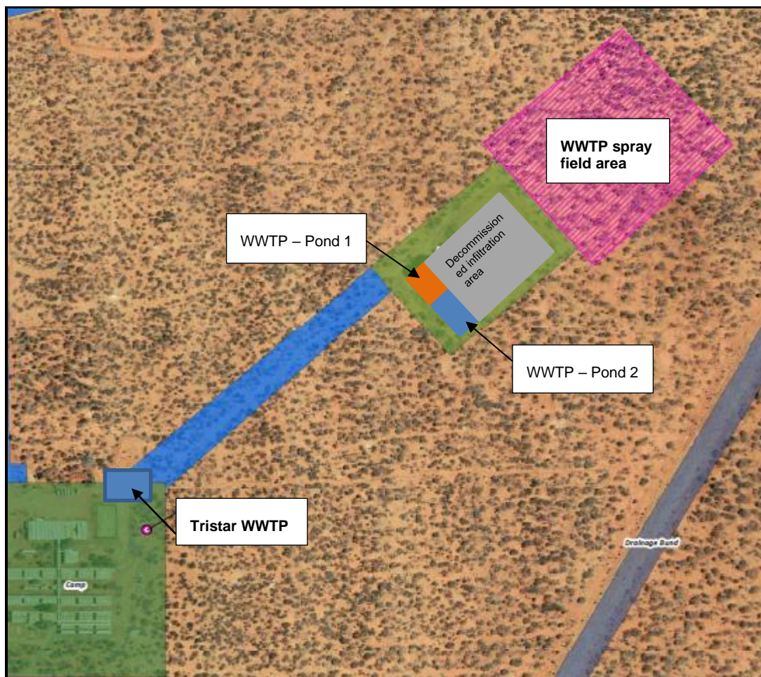
Figure 2: Tristar WWTP, WWTP ponds and spray field area
