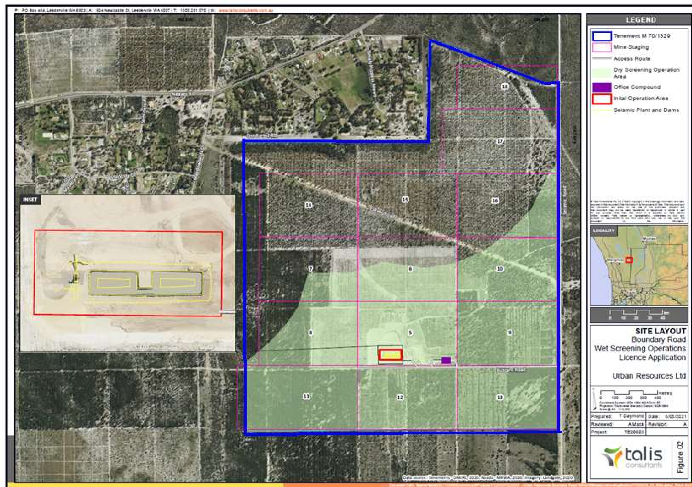
Figure 2: Area for wet screening operation (marked as Initial Operation Area and outlined in red) and settlement ponds
